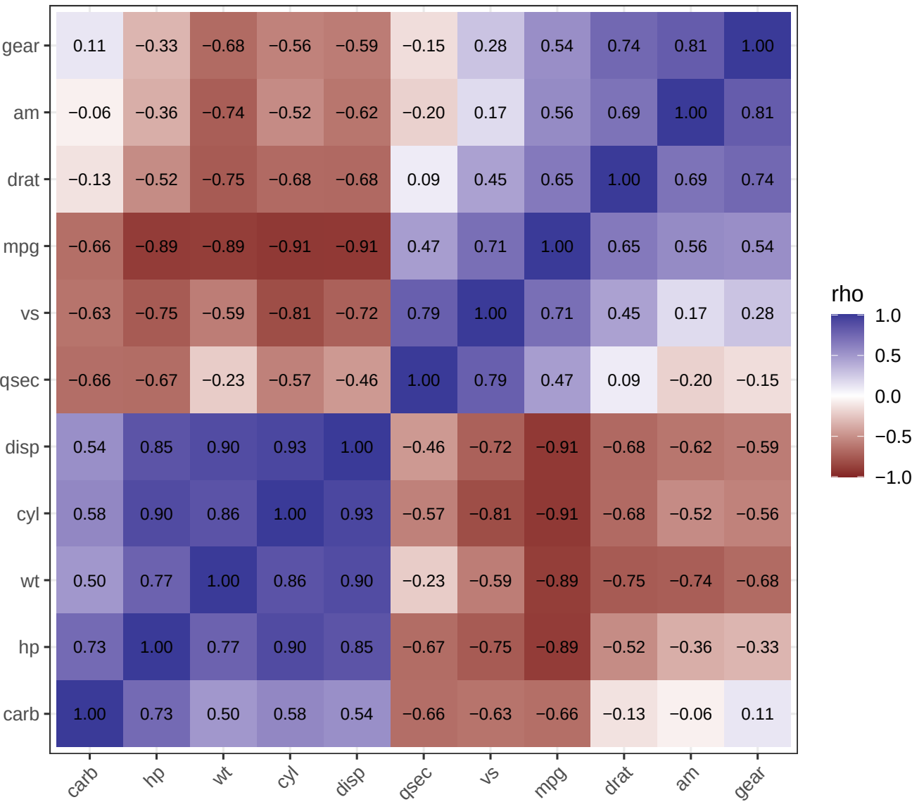
Spearman Correlation (mtcars)
