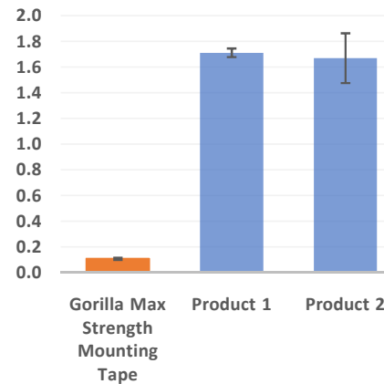
Force to Remove Liner, lbf
