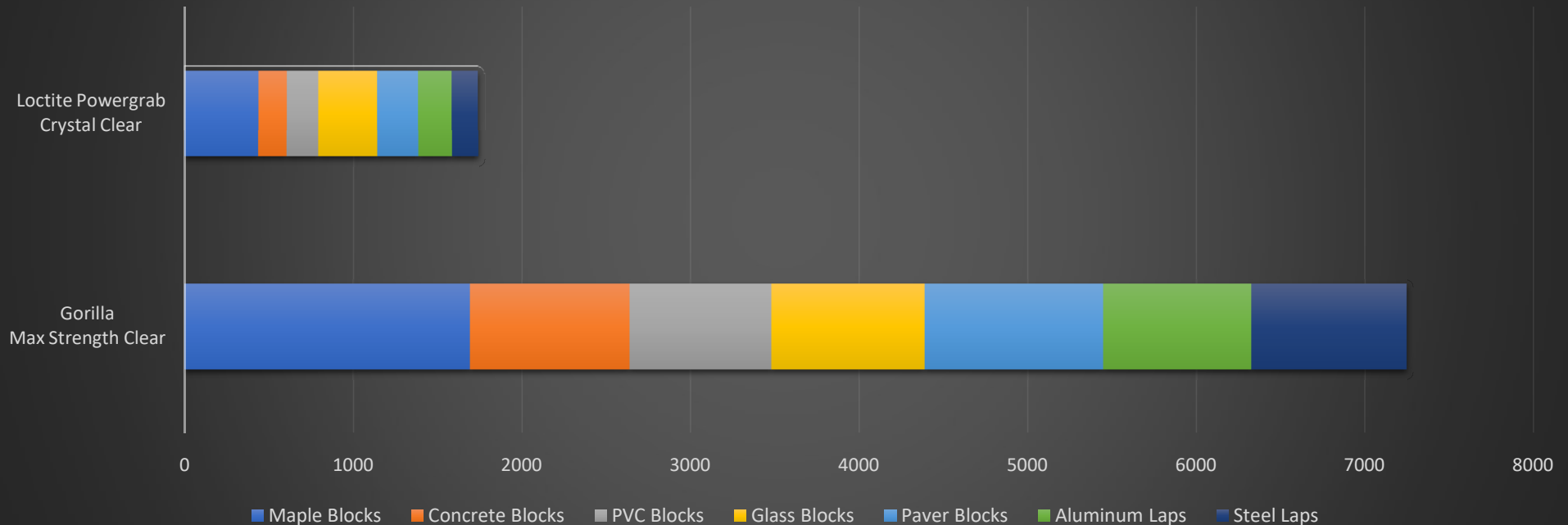
Clear Construction Adhesive Bond Strengths (psi) on Various Substrates
