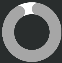
Laravel
