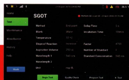
PROGRAMING
