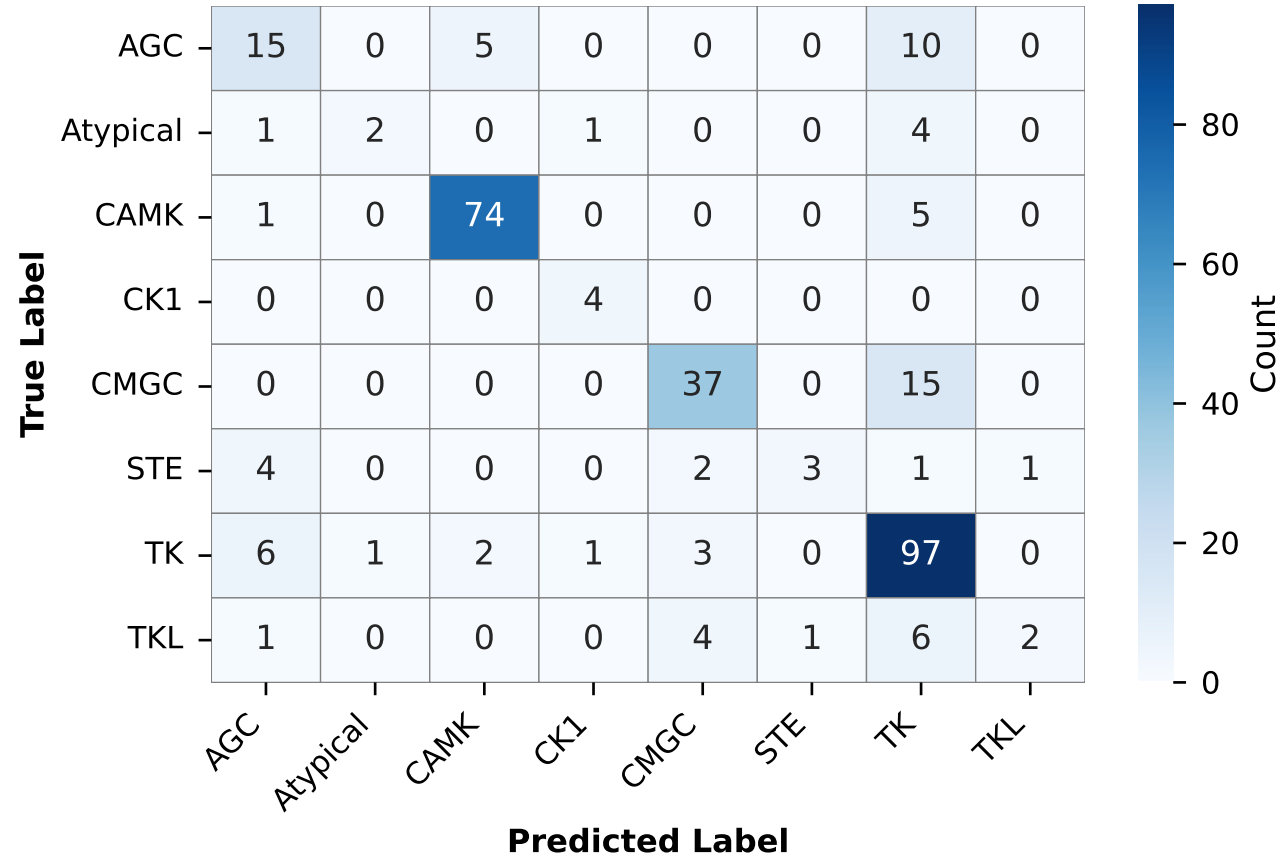
Confusion Matrix (40% Identity Split)
