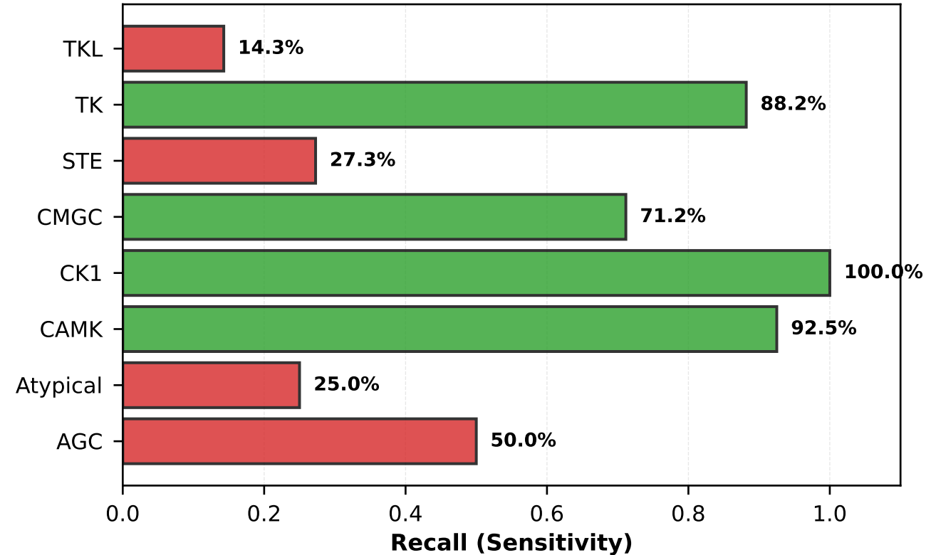
Per-Class Recall (Diagonal Accuracy)
