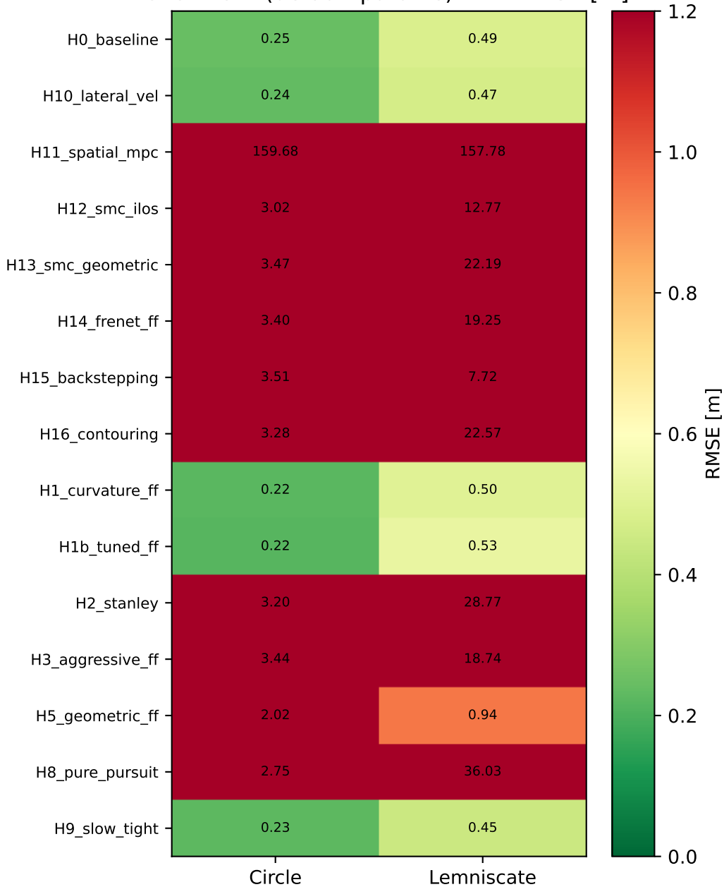
Benchmark (default params): XTE RMSE [m]
