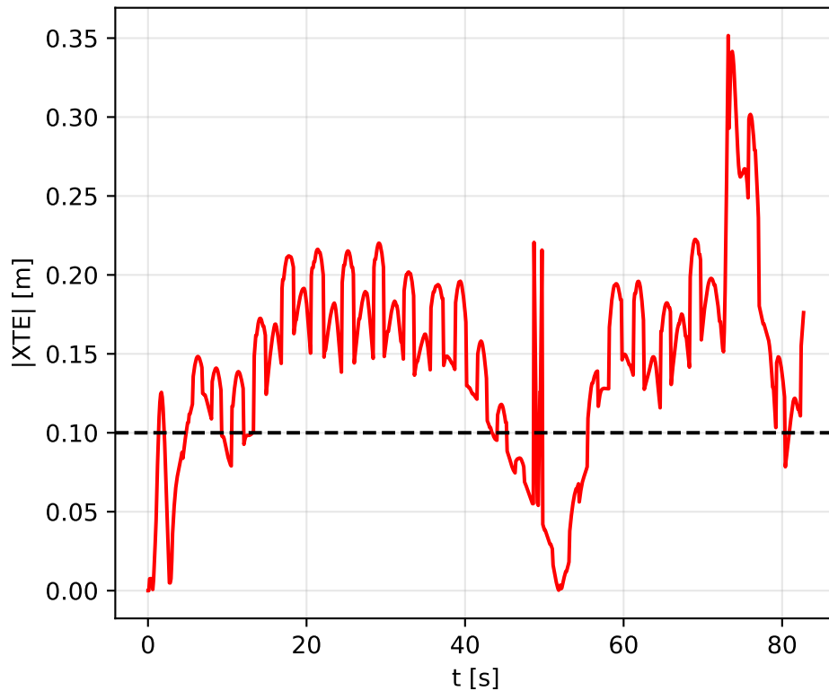
Cross-track error
