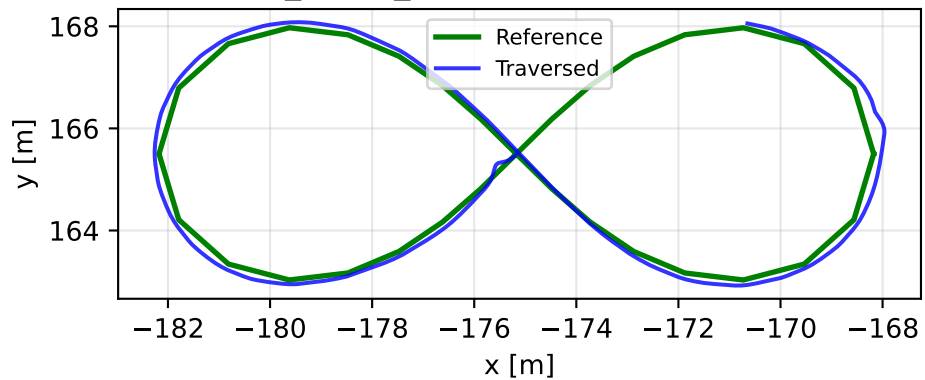
H1b_tuned_ff: trajectory (lemniscate)
