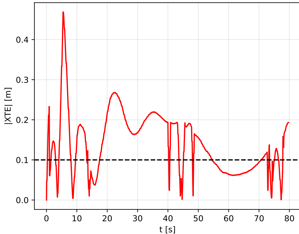
Cross-track error
