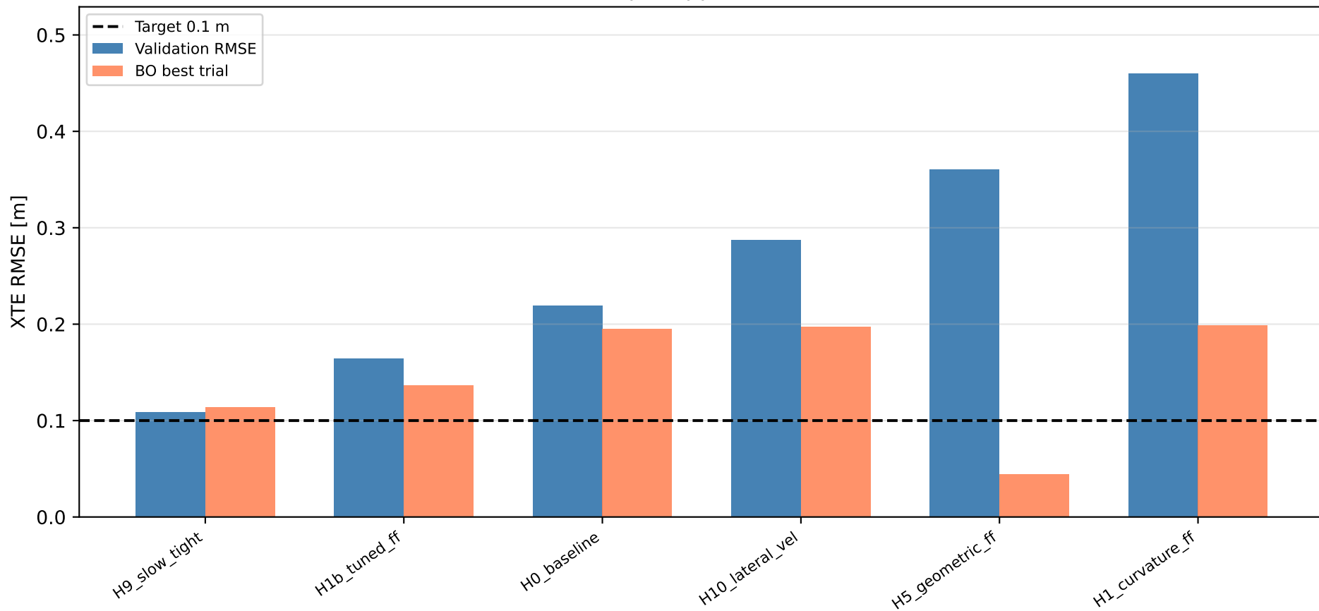
Lemniscate BO: top 6 approaches (28 trials each)
