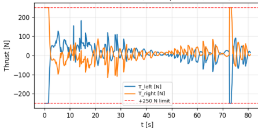
Thruster commands (sat steps: L=24, R=25)
