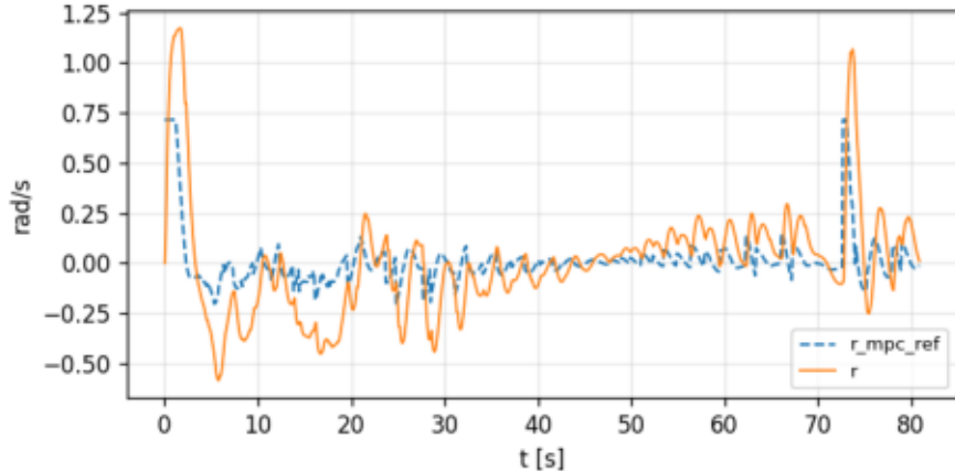
r: MPC ref vs measured
