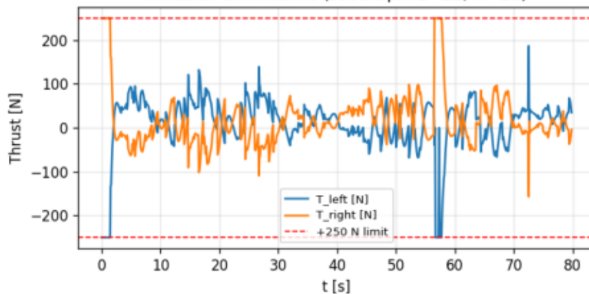
Thruster commands (sat steps: L=22, R=26)
