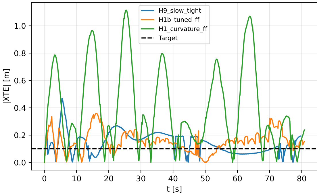
Top BO approaches: XTE time series (lemniscate)
