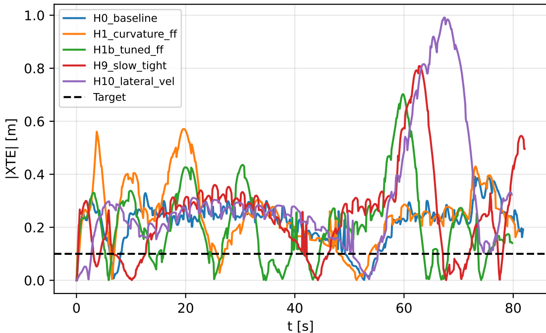
Top-5 approaches: XTE time series (fixed lemniscate)
