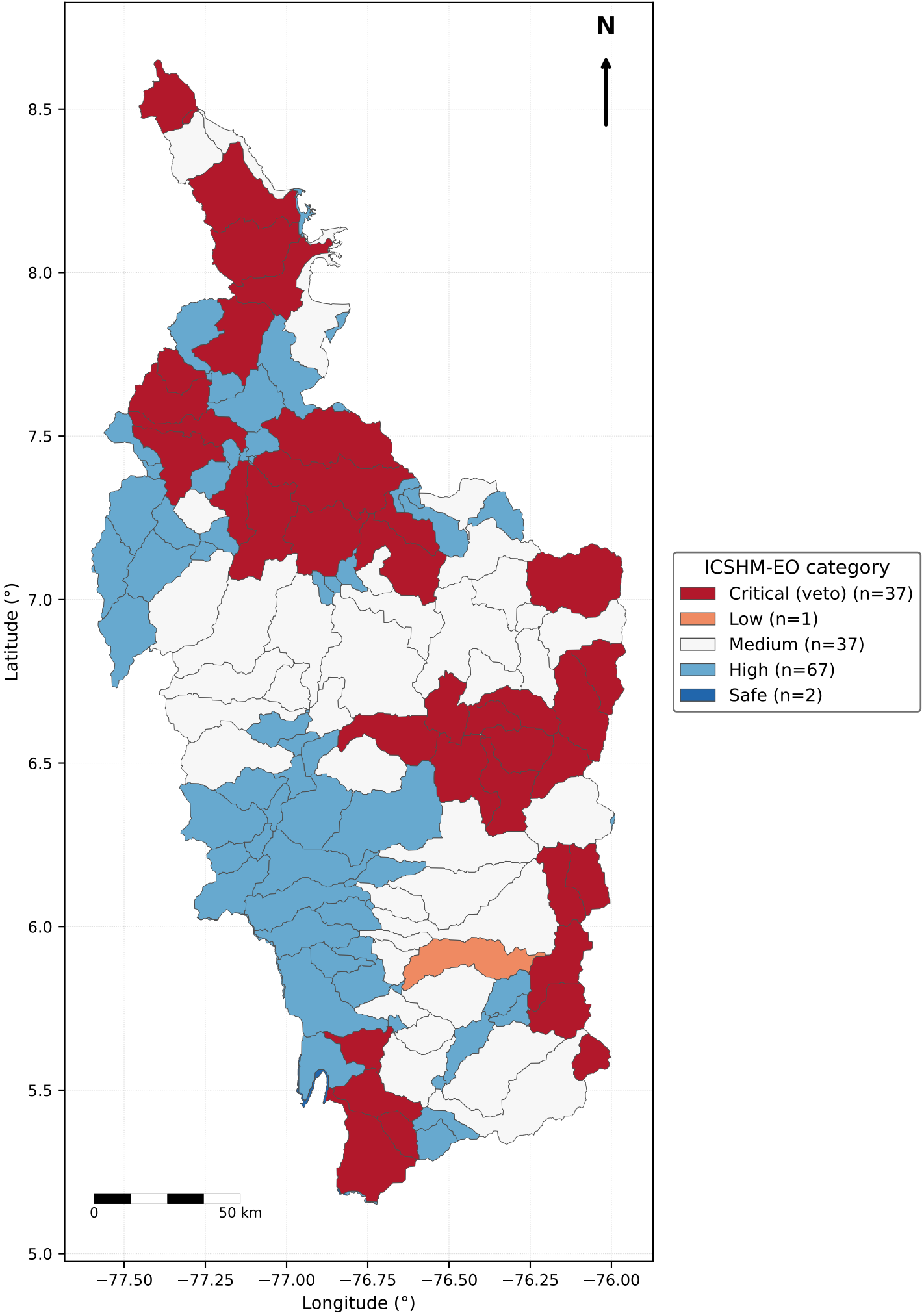
Fig. 3. ICSHM-EO across the Atrato River basin, Colombia (2024).
