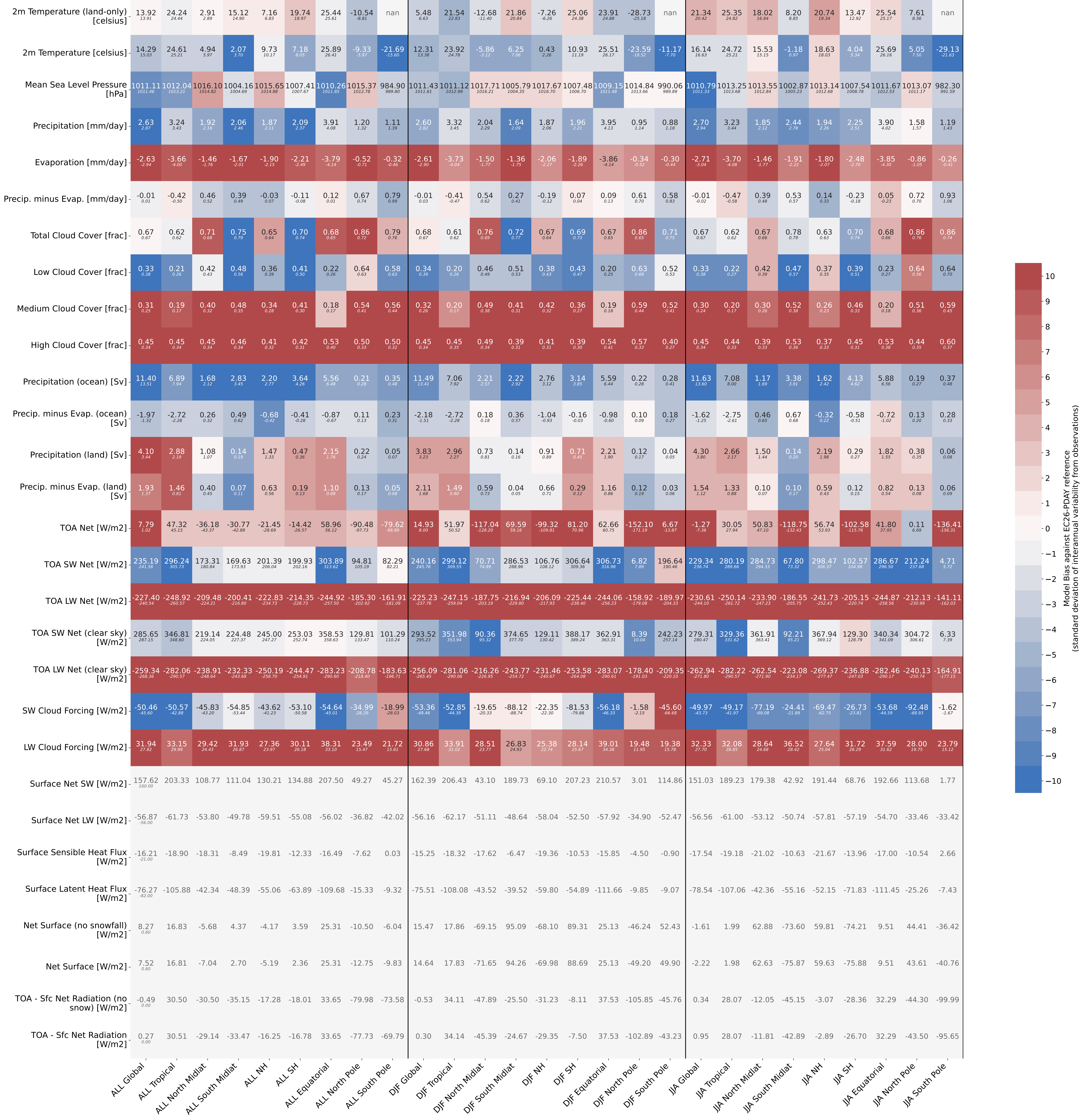
GLOBAL MEAN EC-Earth i024 1990 1992
