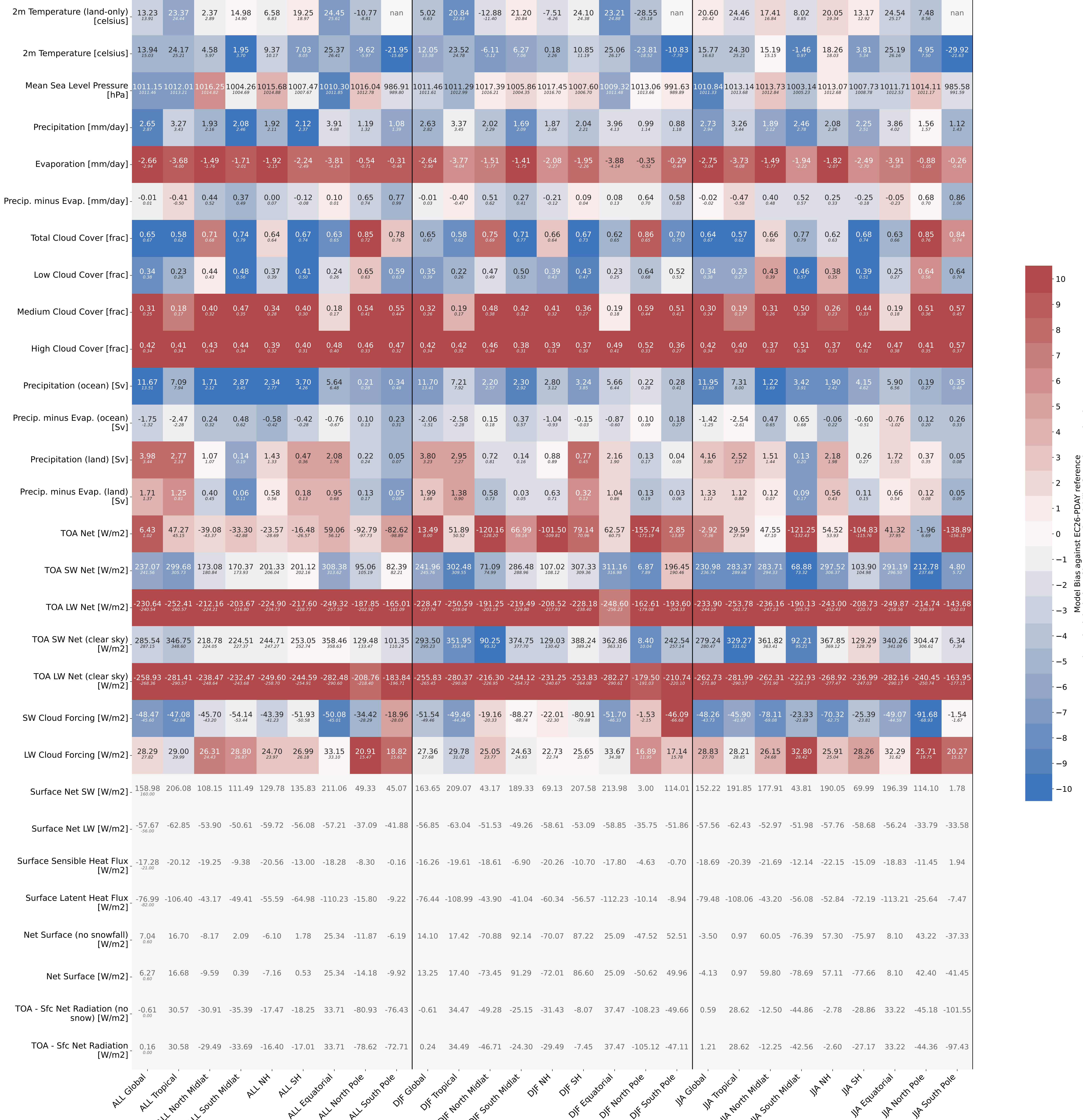
GLOBAL MEAN EC-Earth i029 1990 1992
