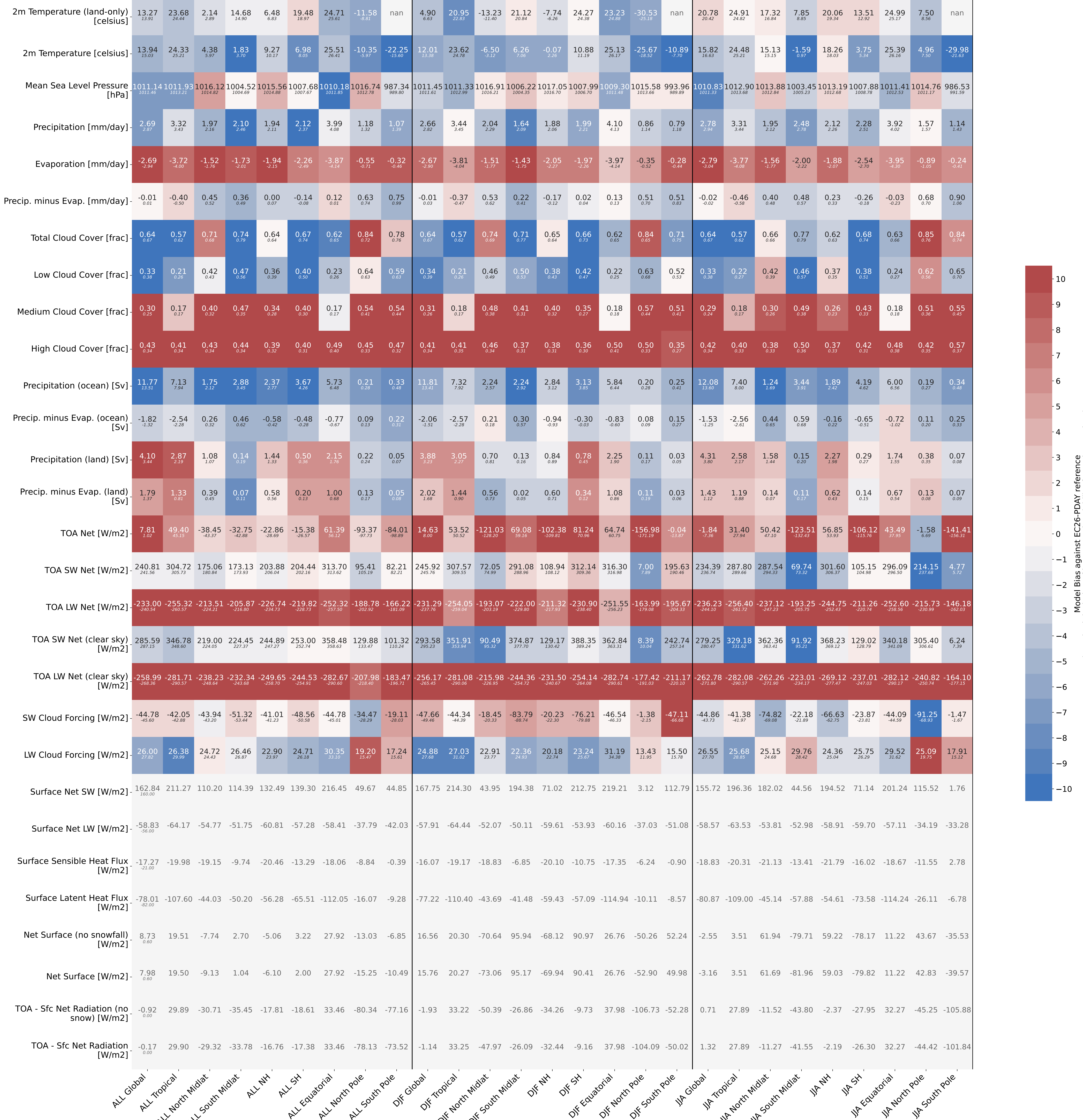
GLOBAL MEAN EC-Earth i039 1990 1992
