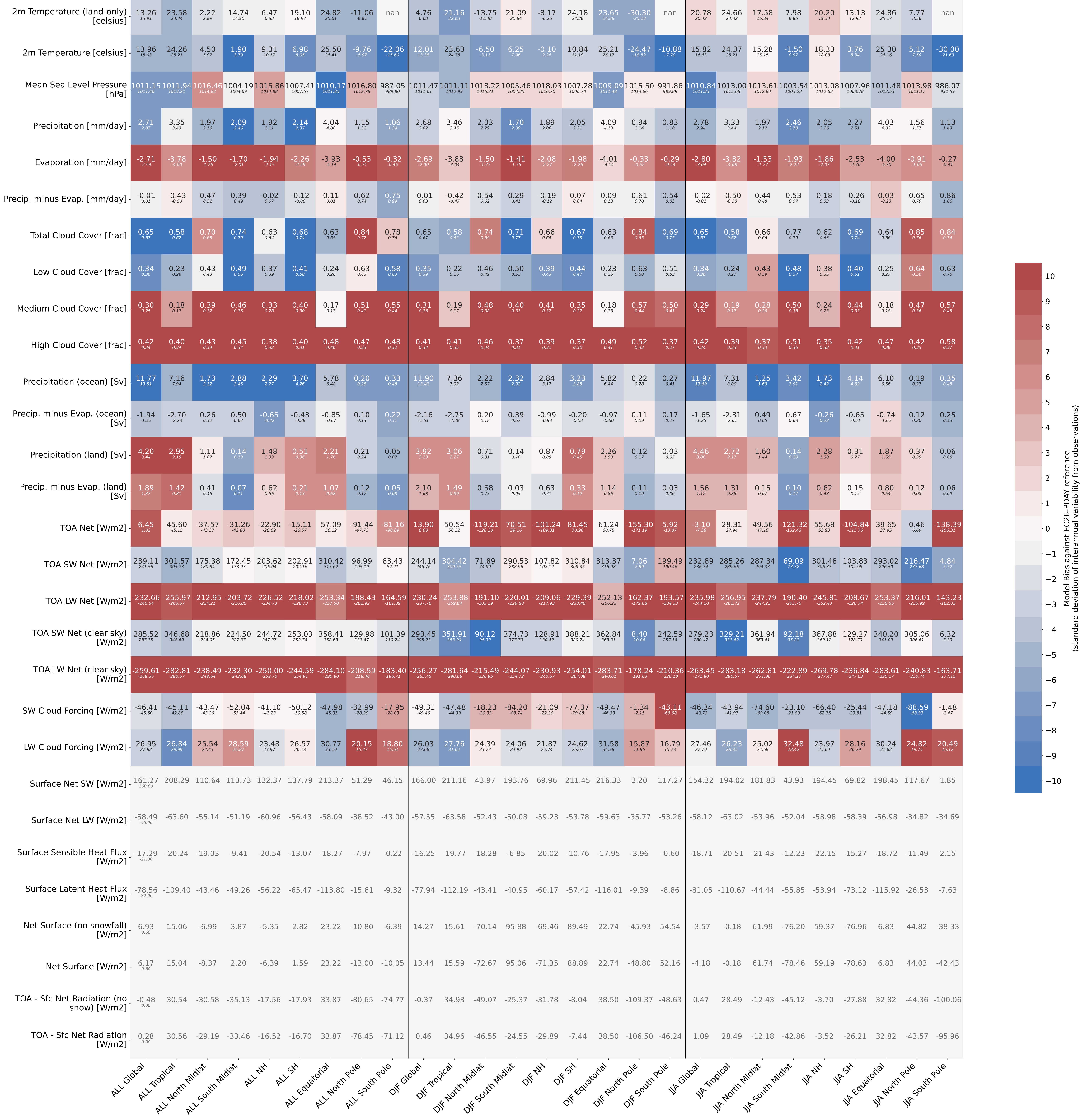
GLOBAL MEAN EC-Earth i058 1990 1992
