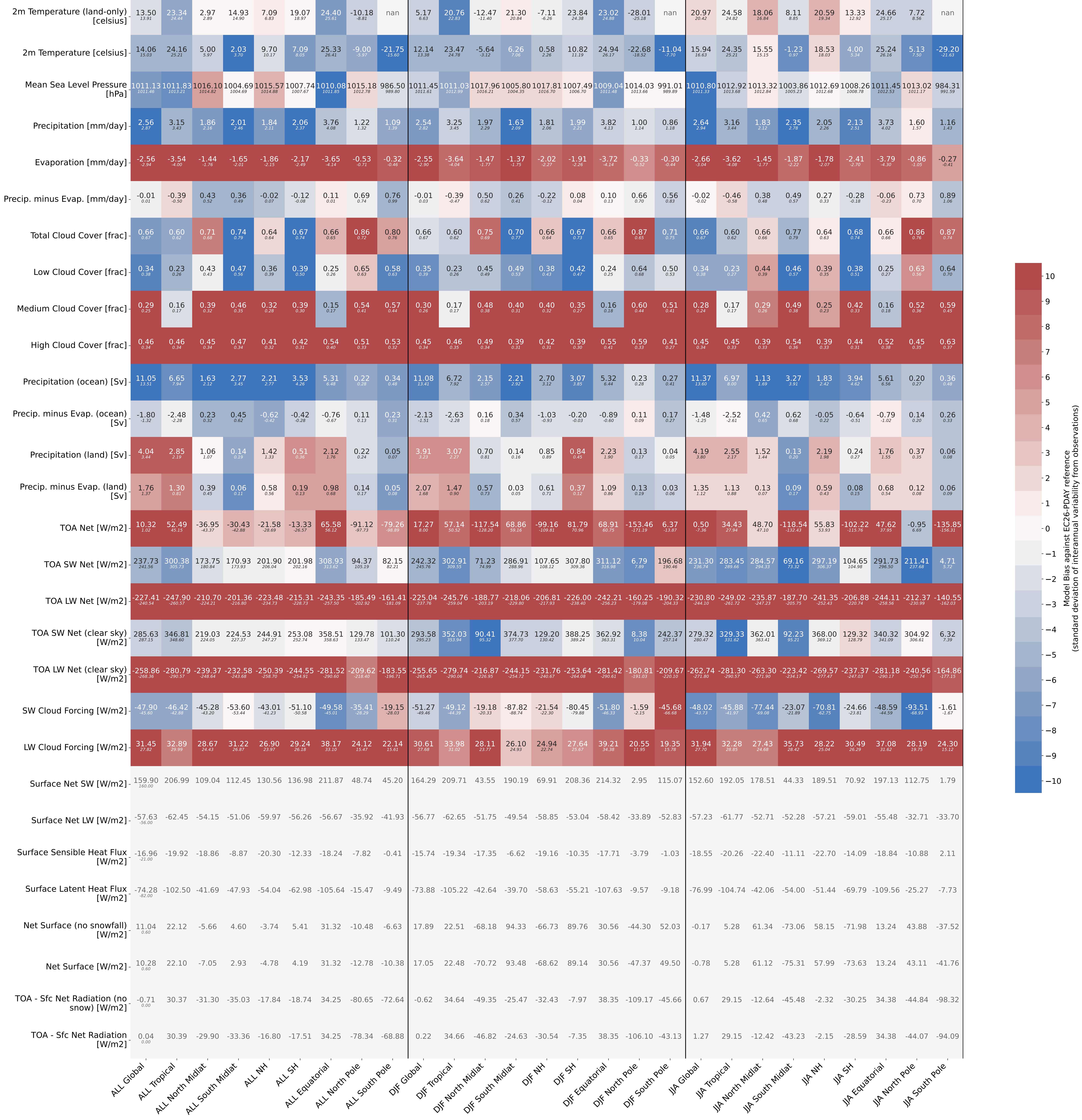
GLOBAL MEAN EC-Earth i069 1990 1992
