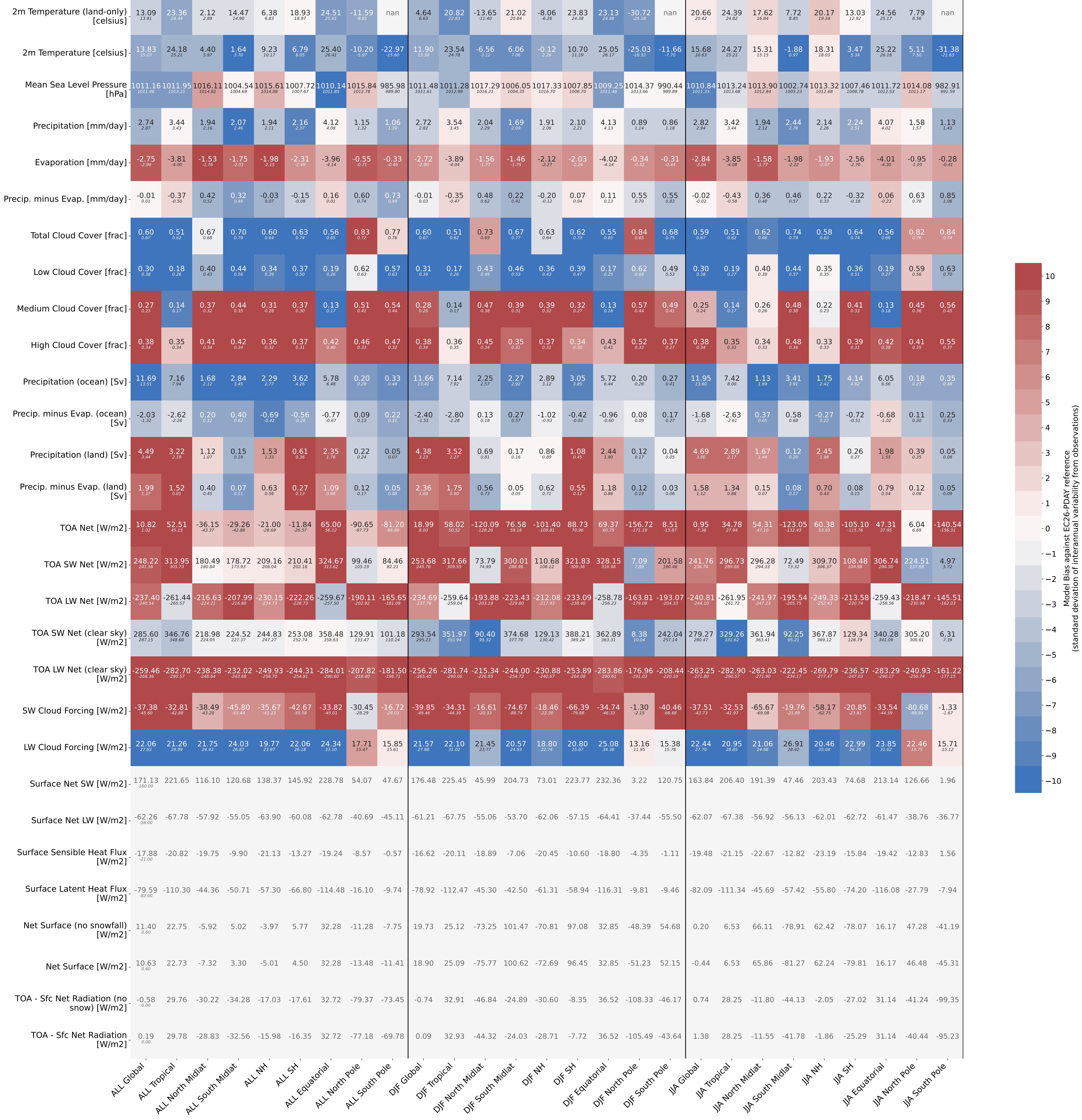
GLOBAL MEAN EC-Earth i077 1990 1992
