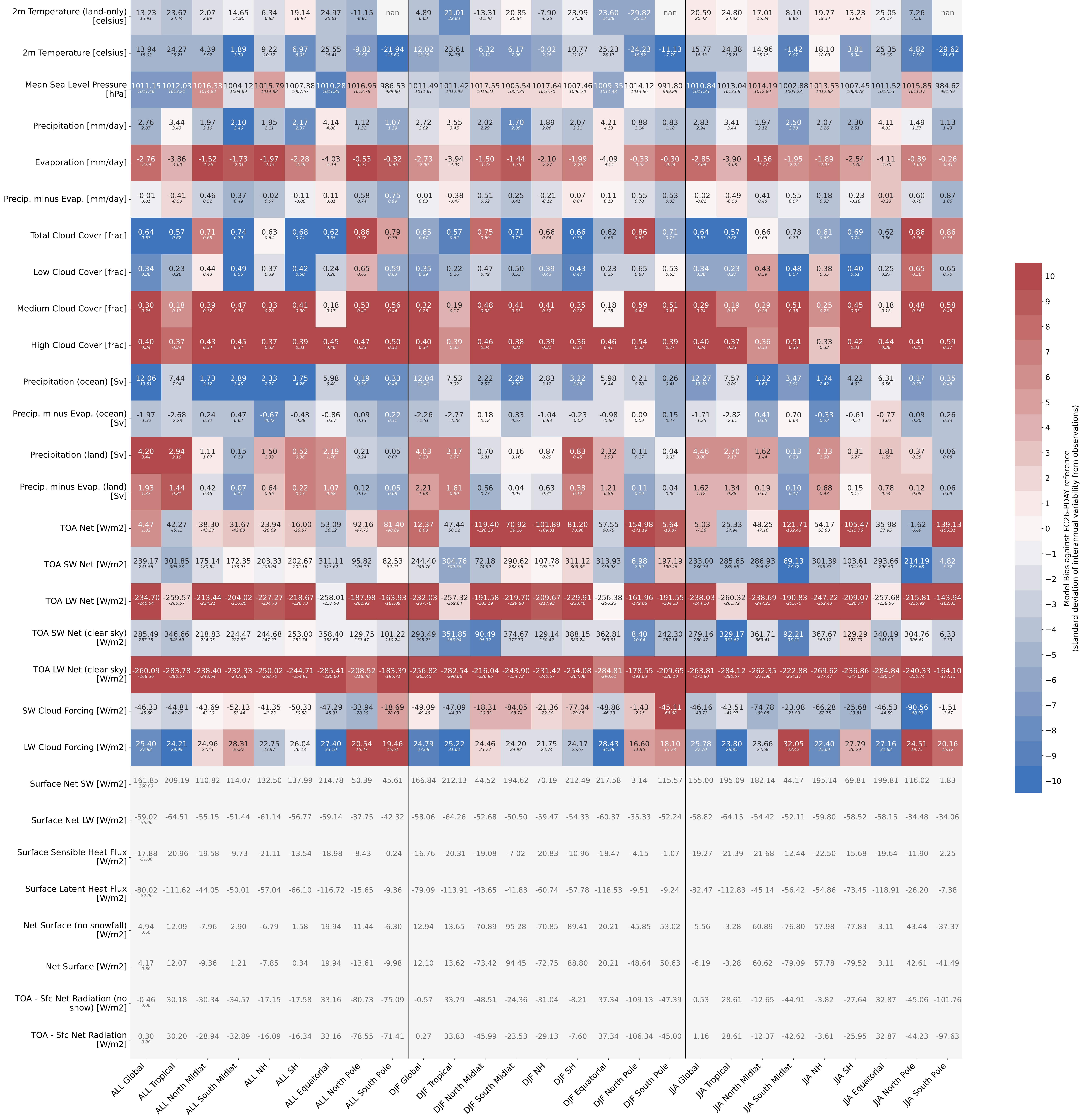
GLOBAL MEAN EC-Earth i078 1990 1992
