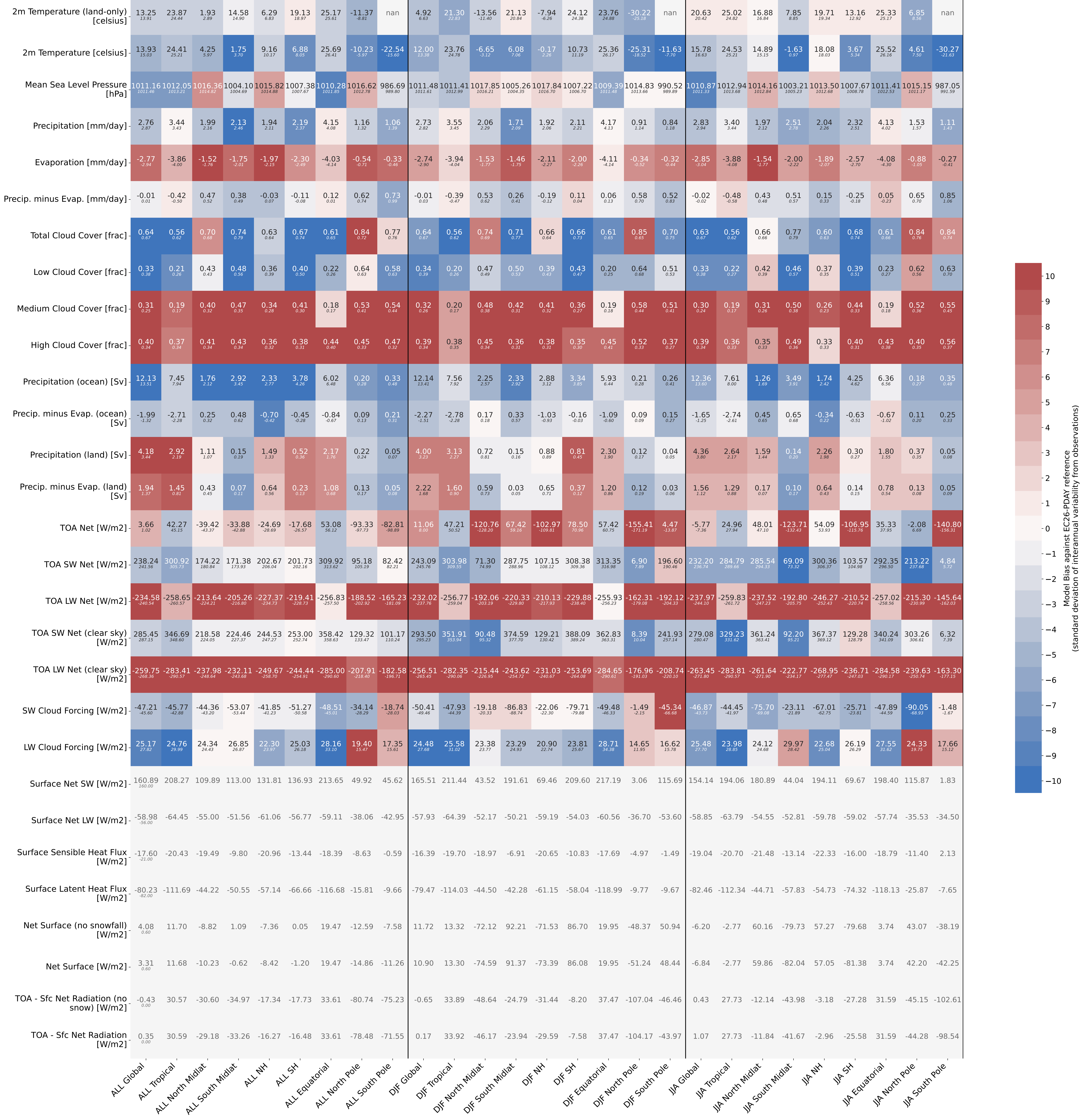
GLOBAL MEAN EC-Earth i080 1990 1992
