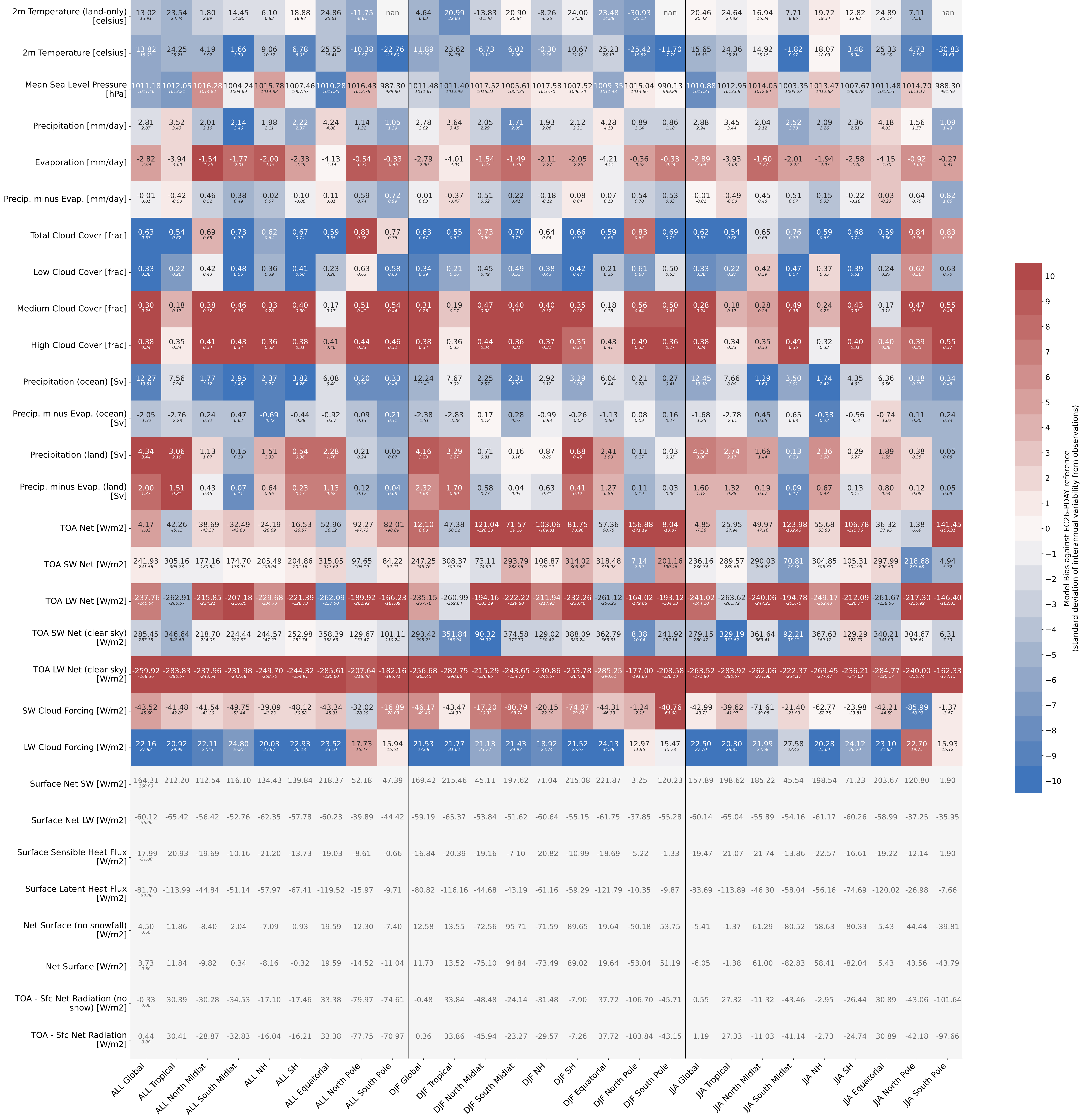
GLOBAL MEAN EC-Earth i090 1990 1992
