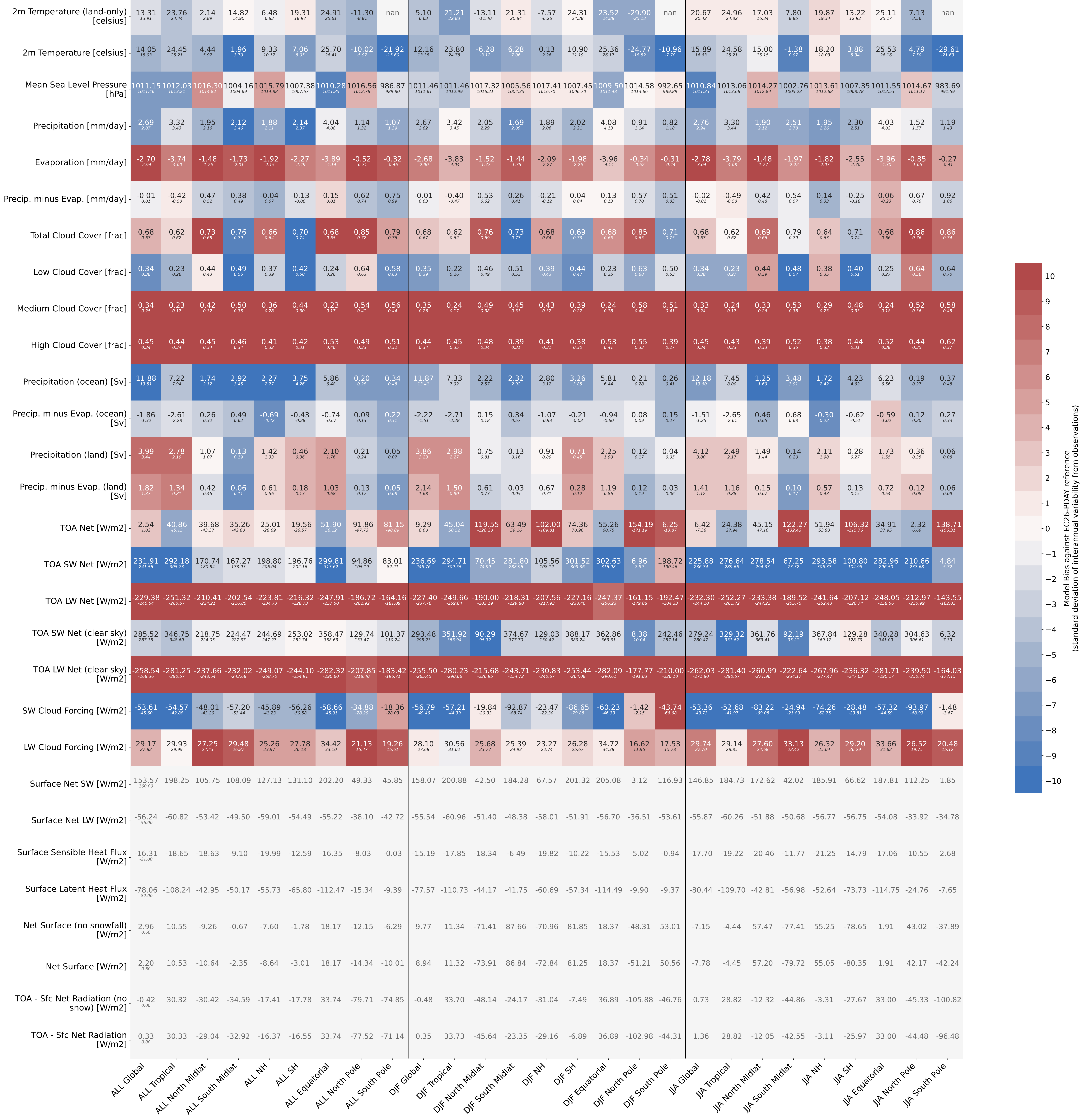
GLOBAL MEAN EC-Earth4 i092 1990 1992
