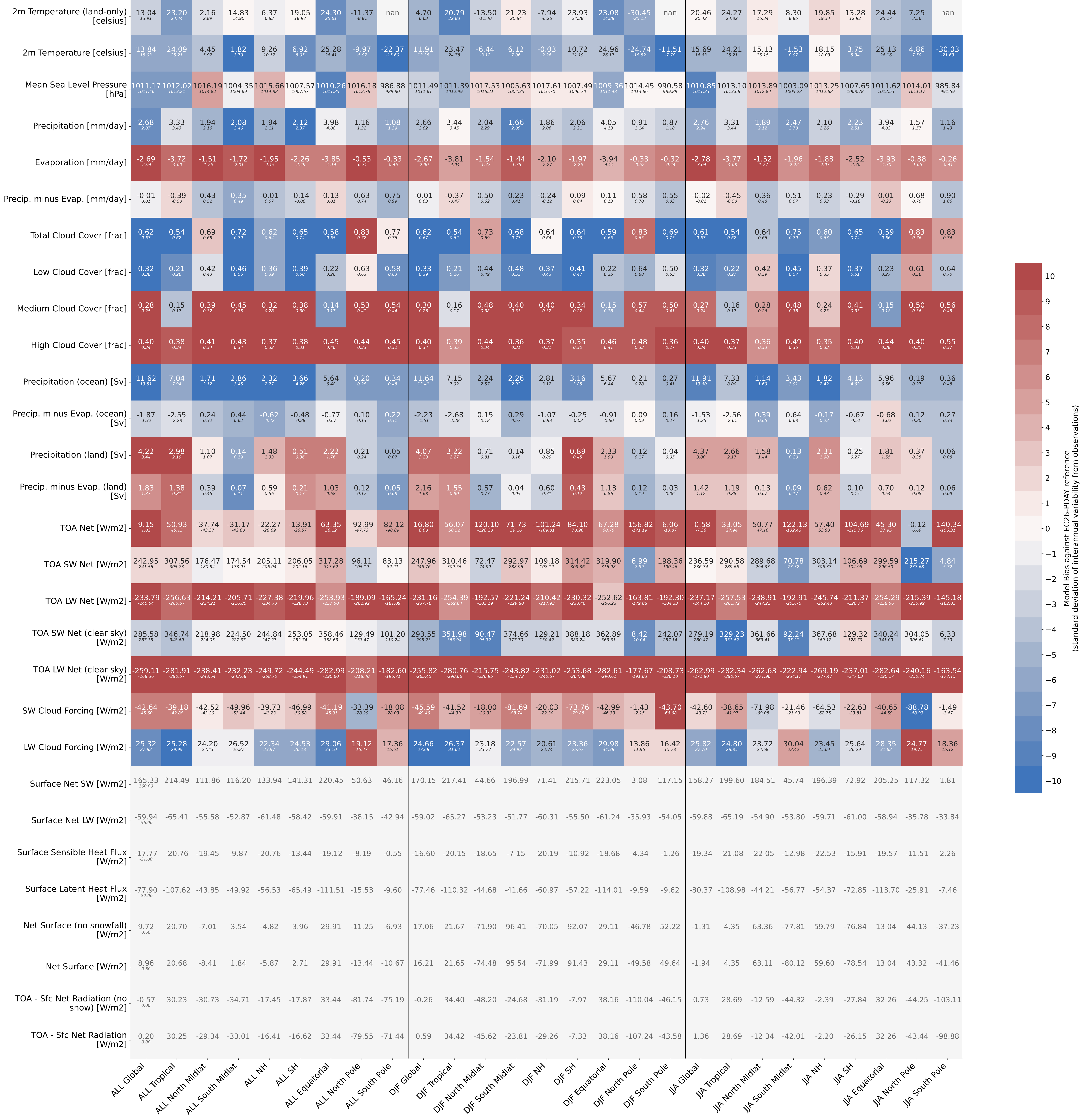
GLOBAL MEAN EC-Earth i093 1990 1992
