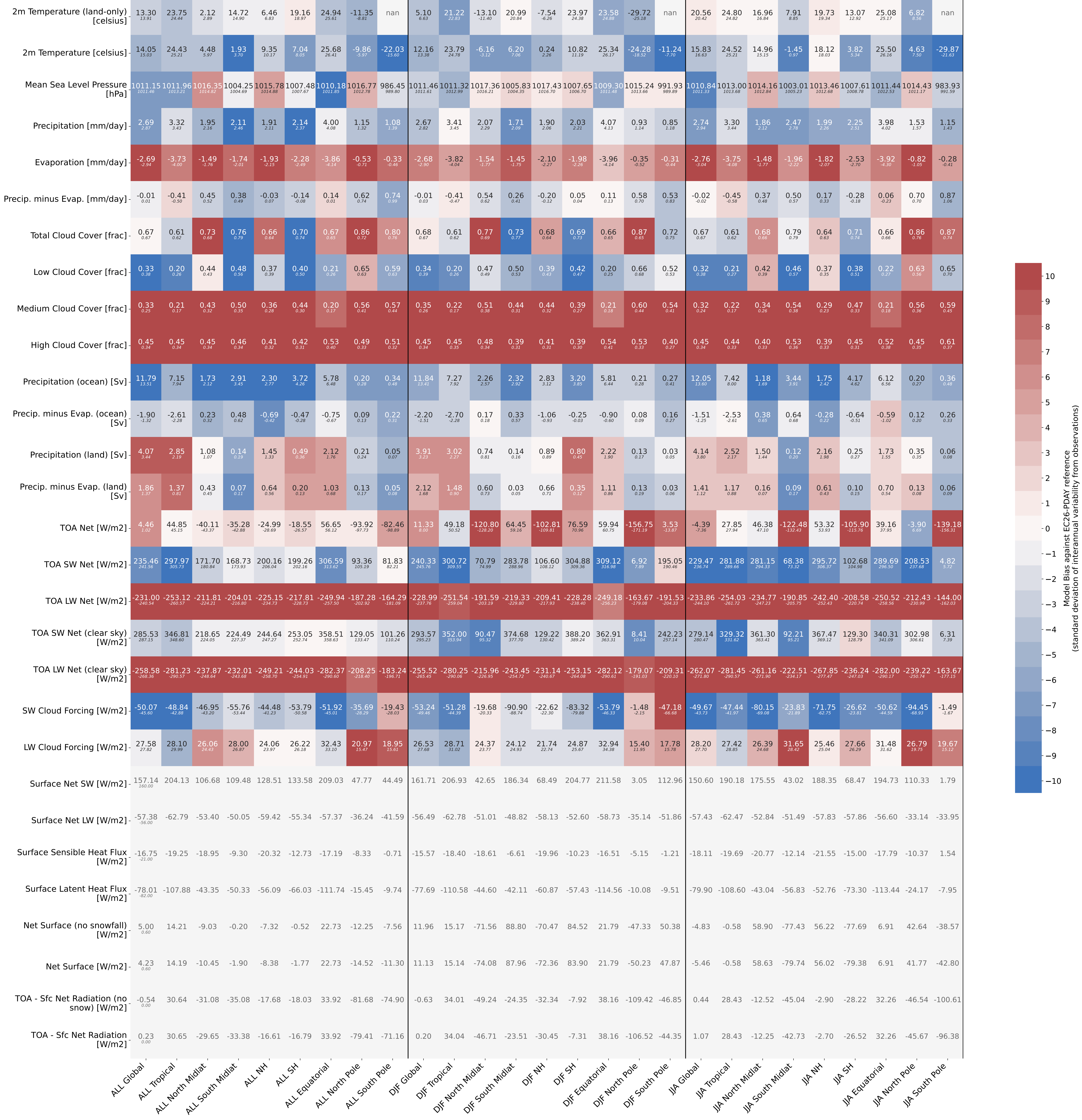
GLOBAL MEAN EC-Earth i099 1990 1992
