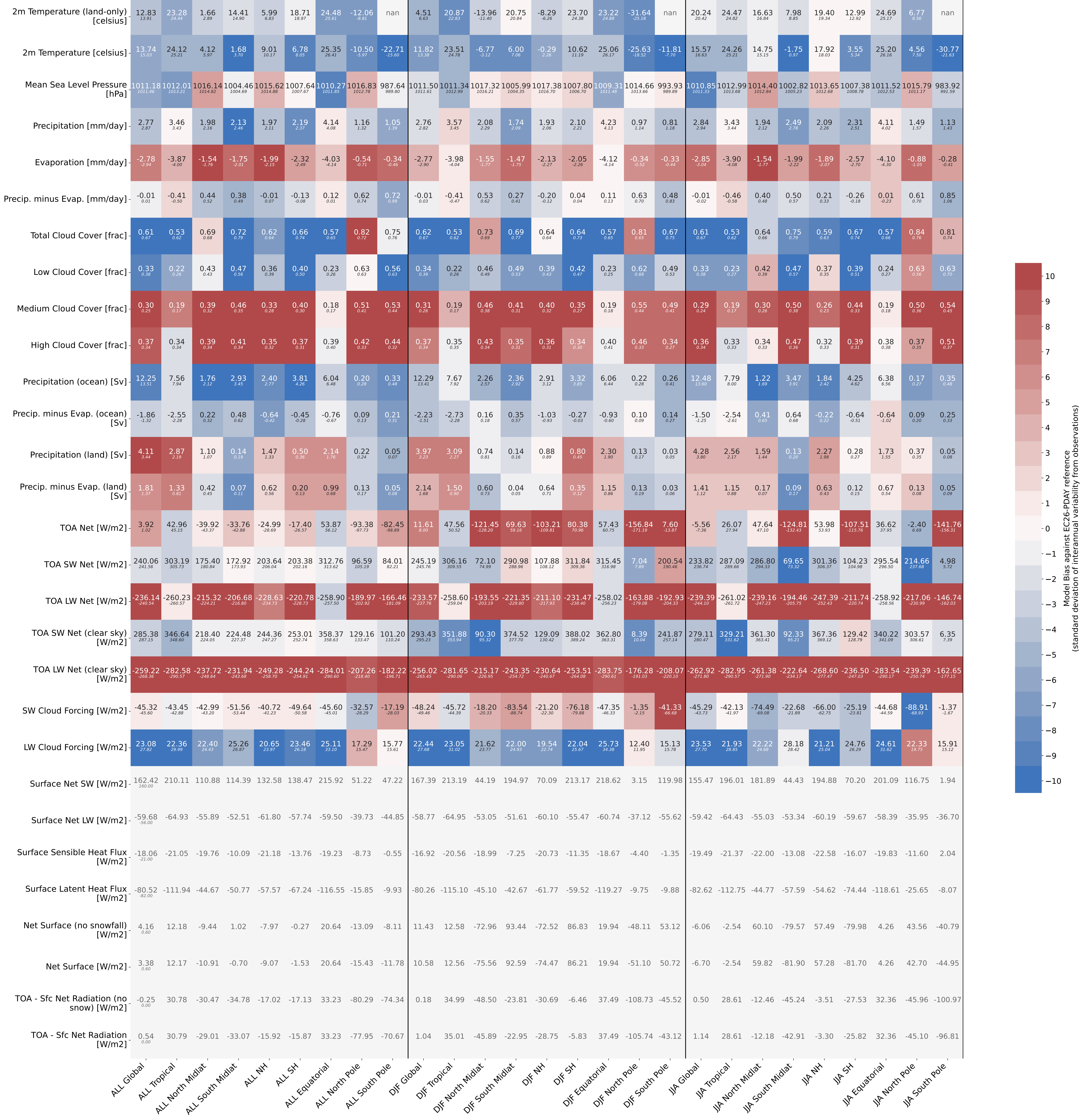
GLOBAL MEAN EC-Earth i026 1991 1992
