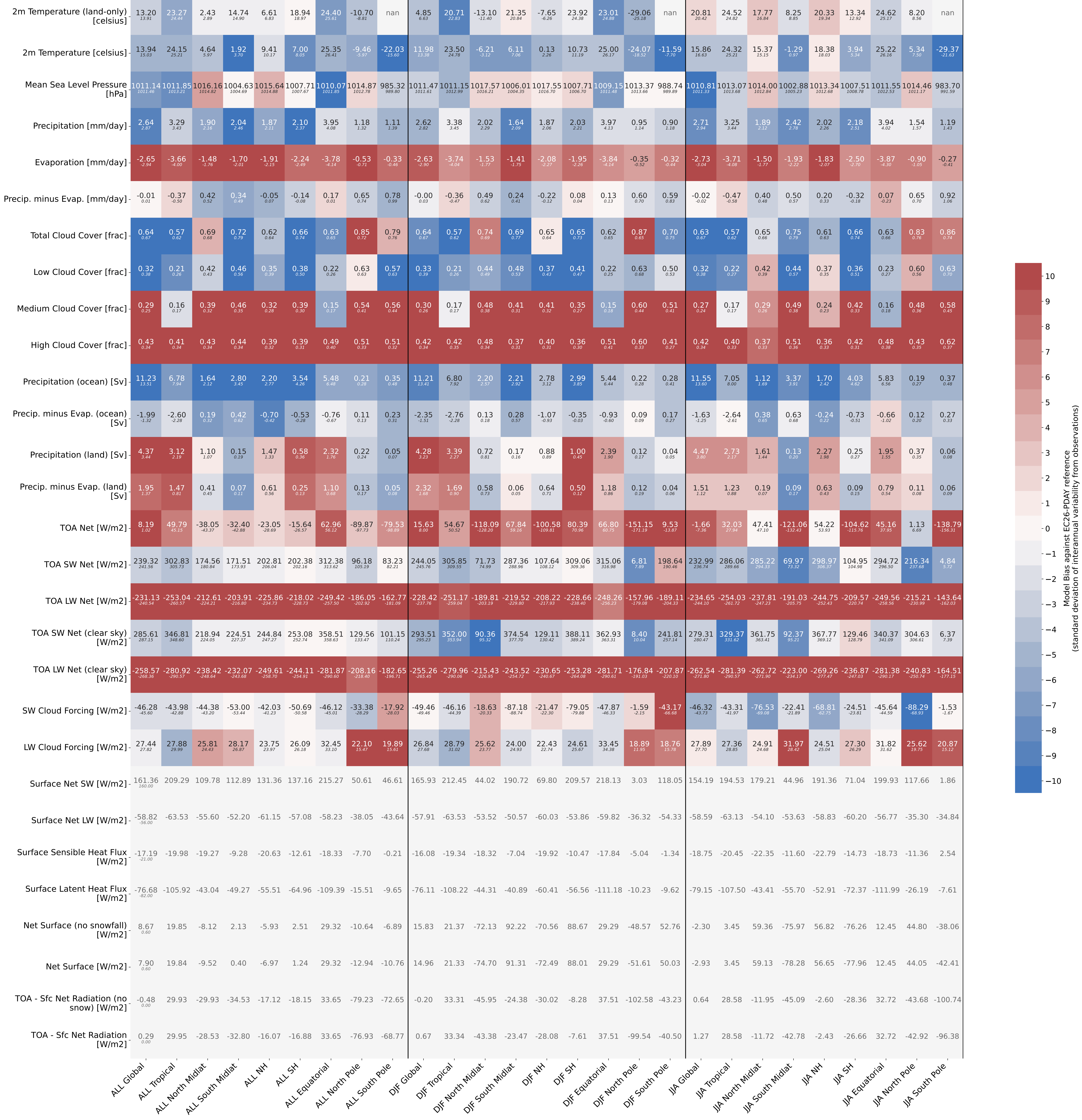
GLOBAL MEAN EC-Earth i047 1991 1992
