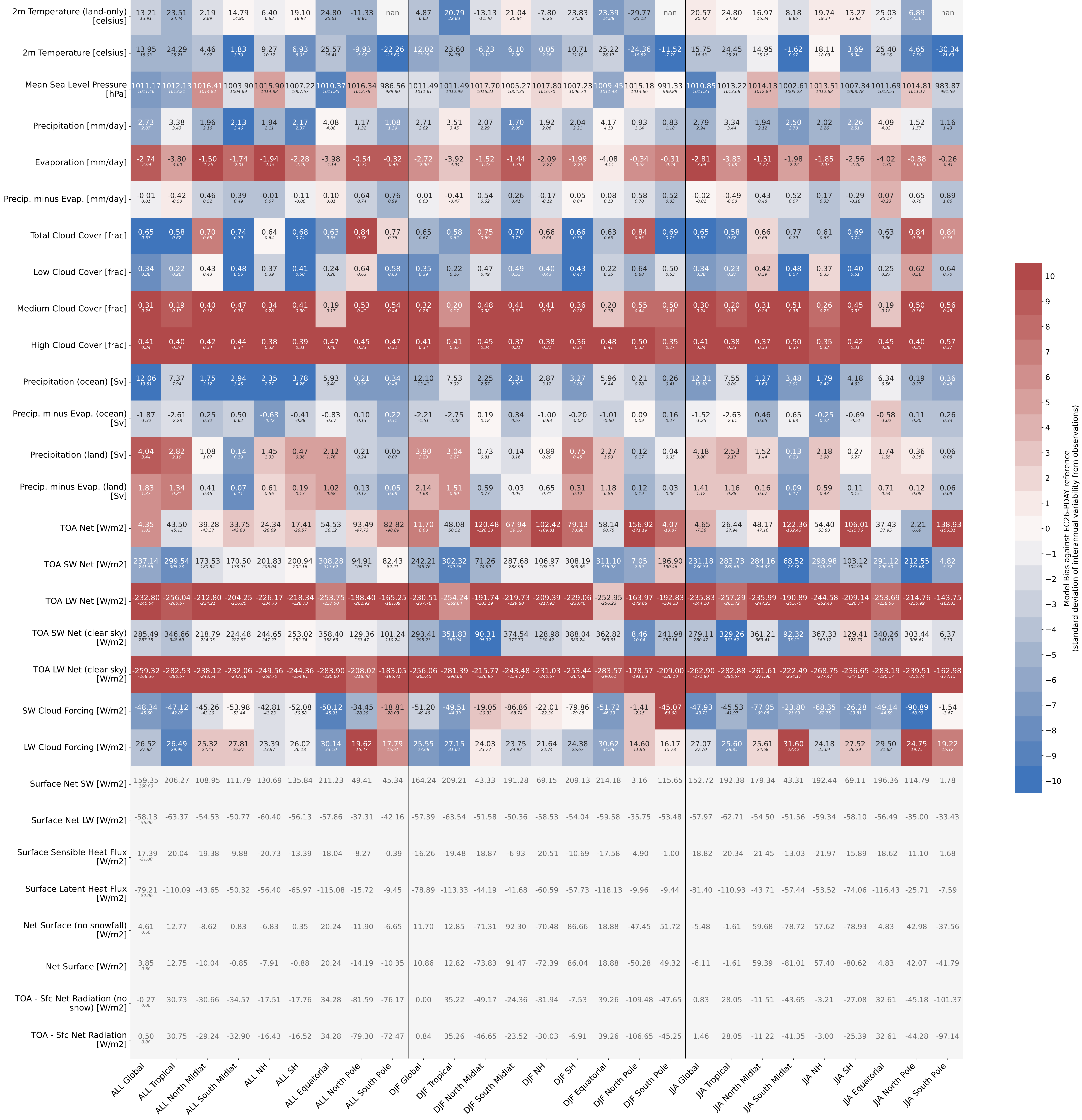
GLOBAL MEAN EC-Earth i048 1991 1992
