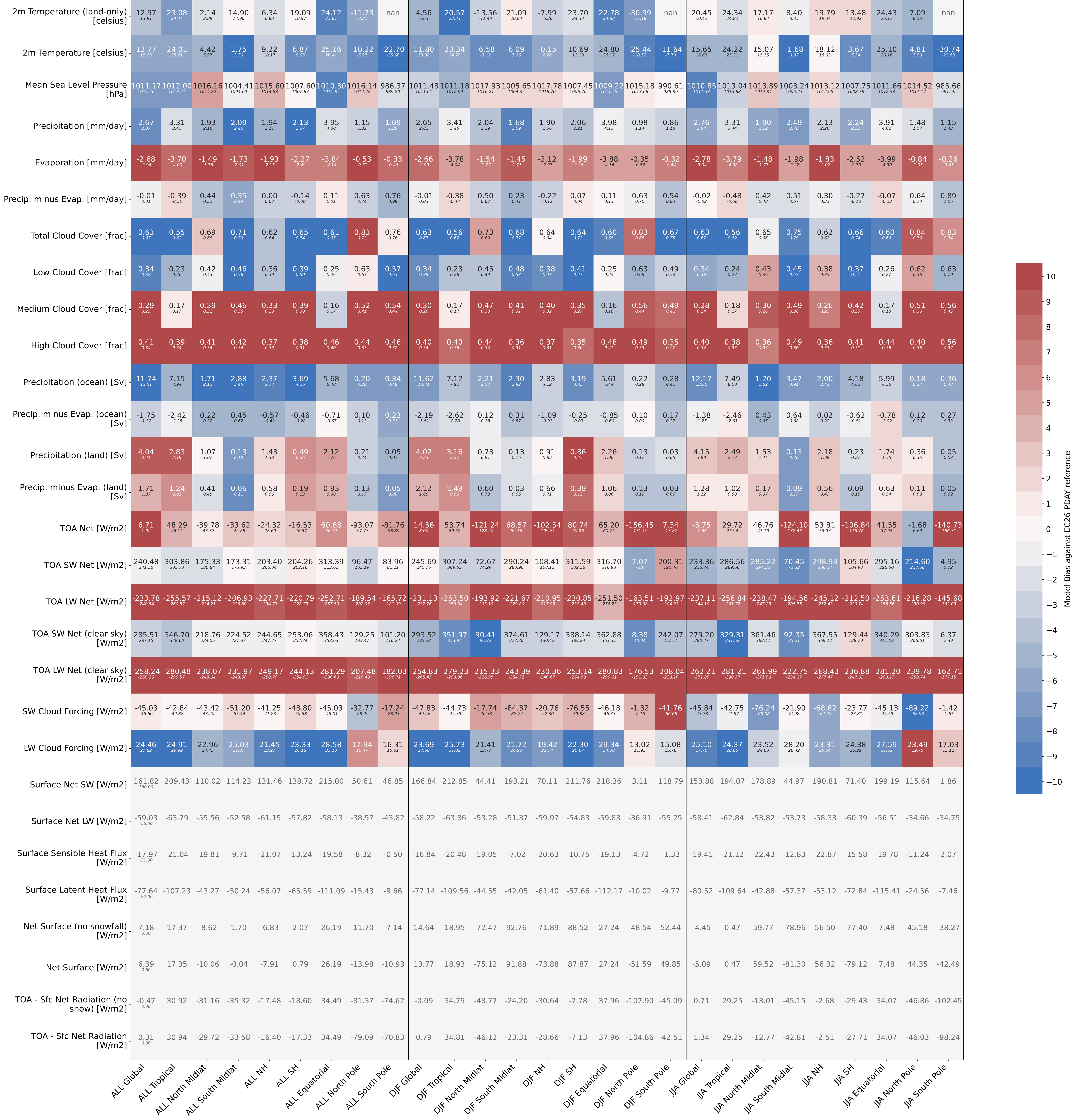
GLOBAL MEAN EC-Earth i079 1991 1992
