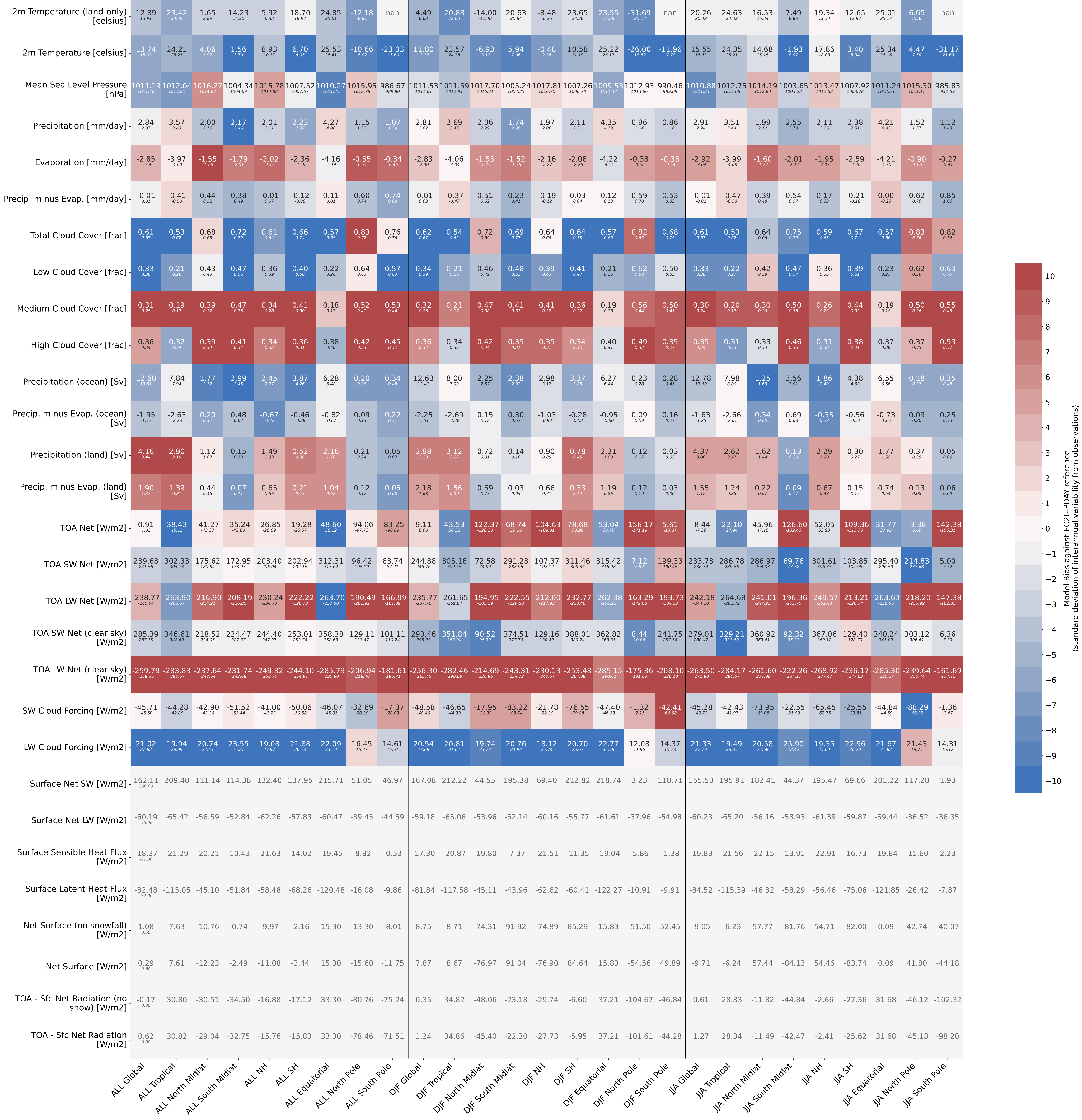
GLOBAL MEAN EC-Earth i106 1991 1992
