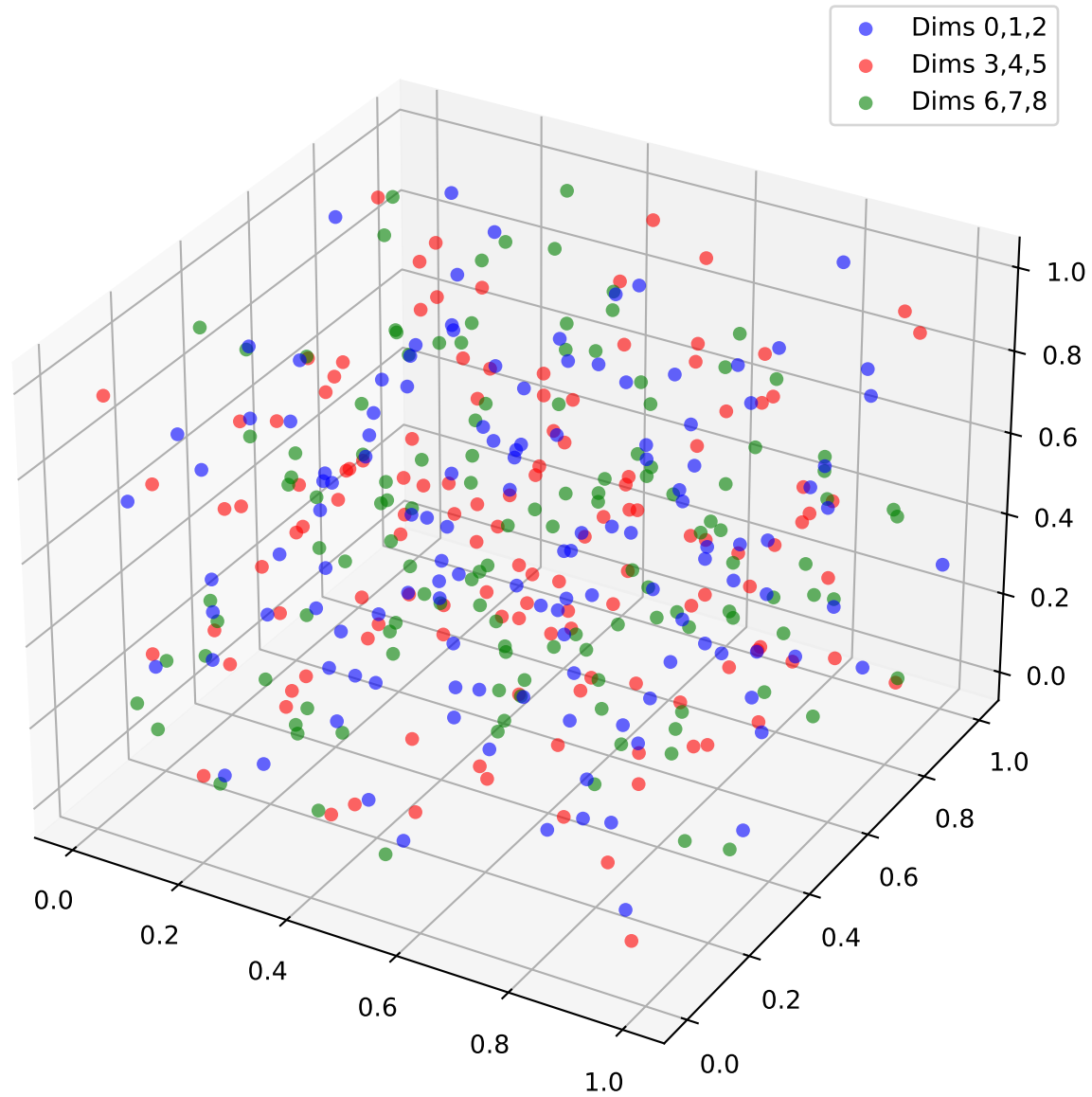
Sobol Space Filling Diagnostic (First 9 Dimensions)
