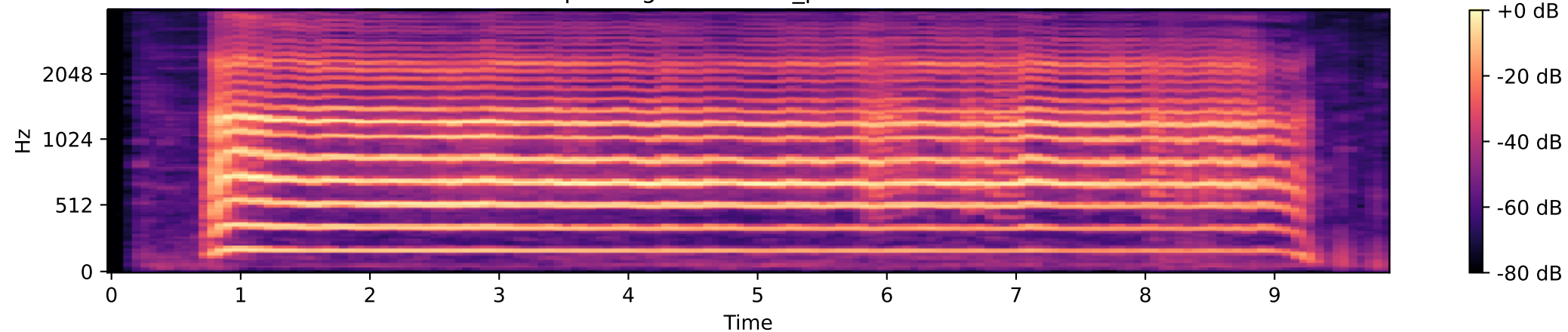
Mel-Spectrogram: ID000_phonationE.wav
