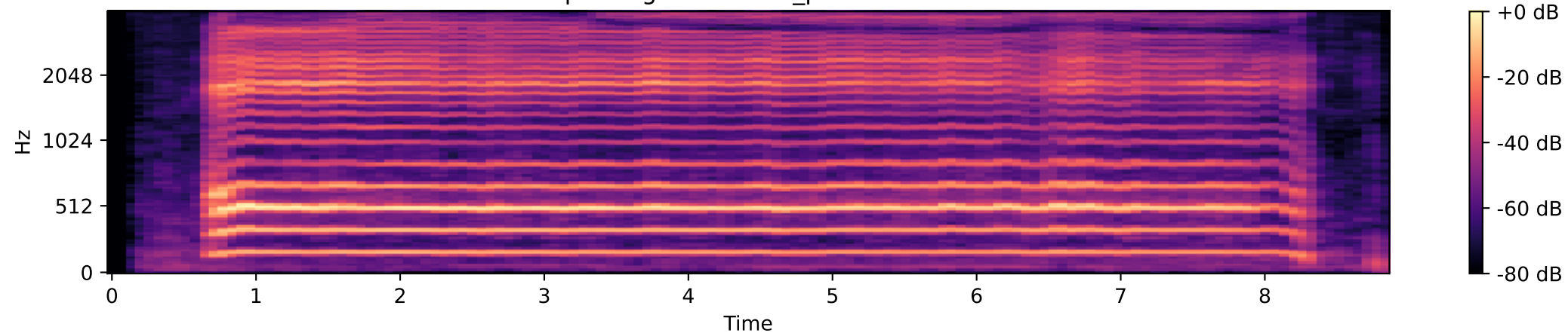
Mel-Spectrogram: ID000_phonationI.wav
