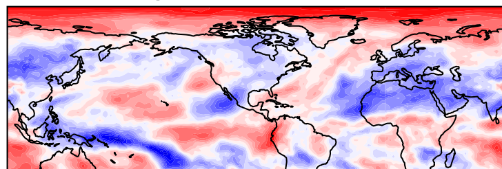
k) OLR SHAP - Winter - Week 4 Greenland High - # Correct cases: 48
