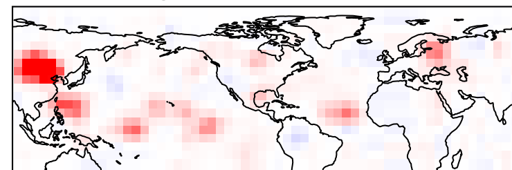
l) OLR SHAP - Winter - Week 6 Greenland High - # Correct cases: 55
