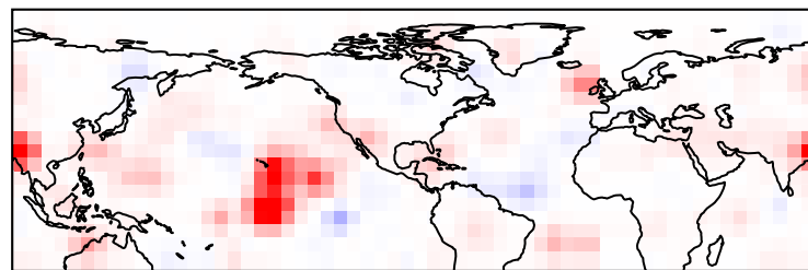
g) OLR Anoms. - Winter - Week 2 Greenland High - # Correct cases: 75
