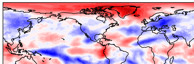
j) OLR SHAP - Winter - Week 2 Greenland High - # Correct cases: 75
