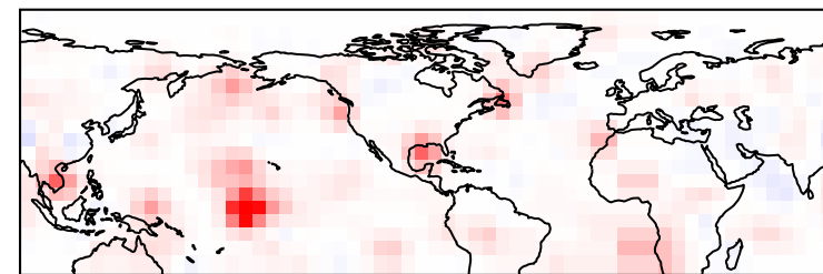
i) OLR Anoms. - Winter - Week 6 Greenland High - # Correct cases: 55
