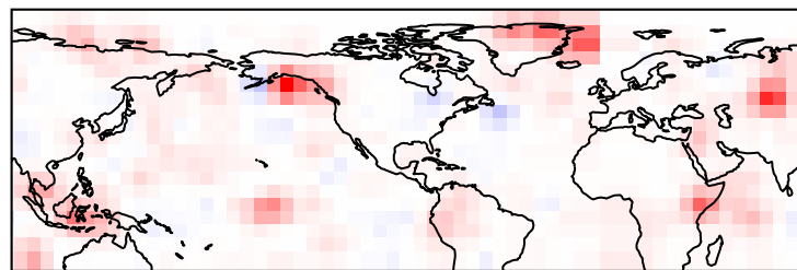
h) OLR Anoms. - Winter - Week 4 Greenland High - # Correct cases: 48
