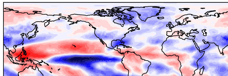
d) OLR SHAP - Winter - Week 5 Pacific Trough - # Correct cases: 126
