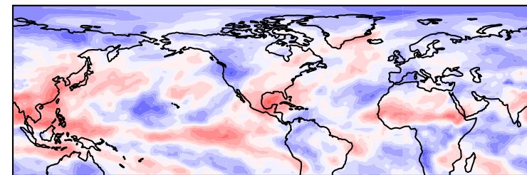
f) OLR SHAP - Fall - Week 5 Pacific Ridge - # Correct cases: 82
