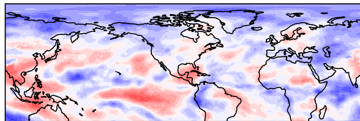
e) OLR SHAP - Fall - Week 3 Pacific Ridge - # Correct cases: 74
