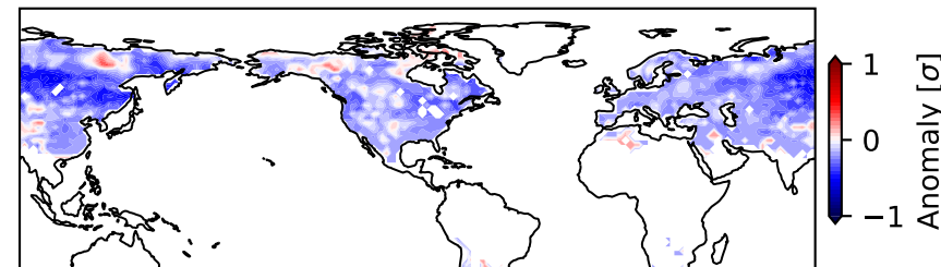
f) SD SHAP - Fall - Week 6 Pacific Ridge - # Correct cases: 114
