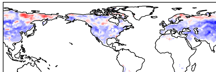
e) SD SHAP - Fall - Week 3 Pacific Ridge - # Correct cases: 88
