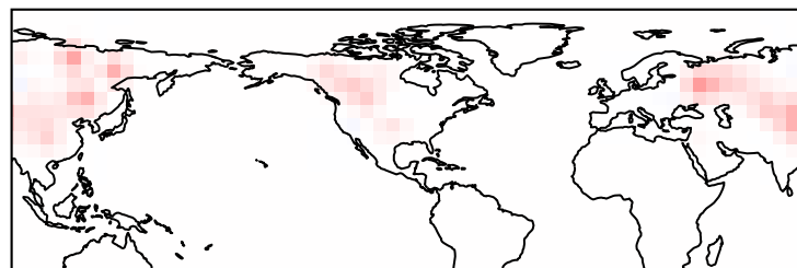
h) SD Anoms. - Winter - Week 7 Greenland High - # Correct cases: 47
