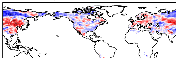
g) SD Anoms. - Winter - Week 4 Greenland High - # Correct cases: 43
