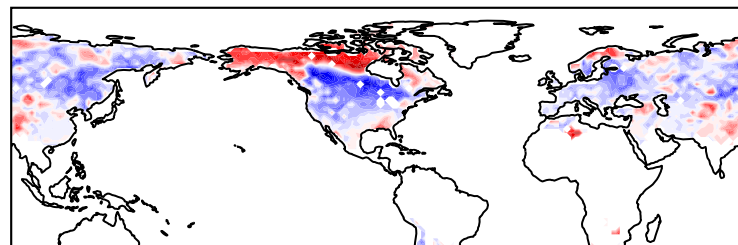
d) SD SHAP - Spring - Week 3 Pacific Trough - # Correct cases: 109
