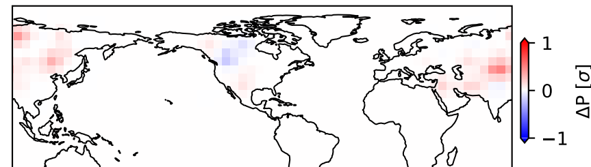
i) SD Anoms. - Fall - Week 6 Greenland High - # Correct cases: 56
