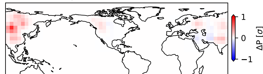
l) SD SHAP - Fall - Week 6 Greenland High - # Correct cases: 56
