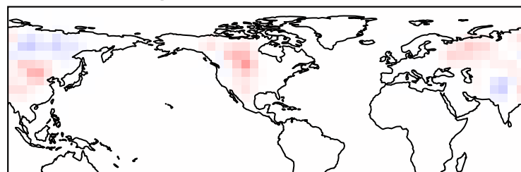
j) SD SHAP - Winter - Week 4 Greenland High - # Correct cases: 43
