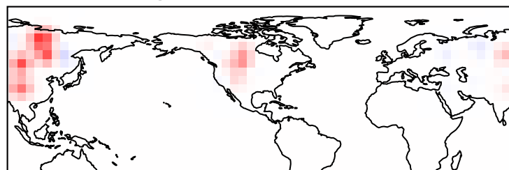
k) SD SHAP - Winter - Week 7 Greenland High - # Correct cases: 47
