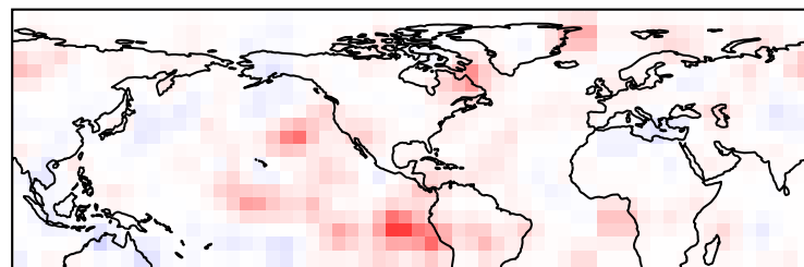
g) U200 Anoms. - Fall - Week 6 Pacific Trough - # Correct cases: 87
