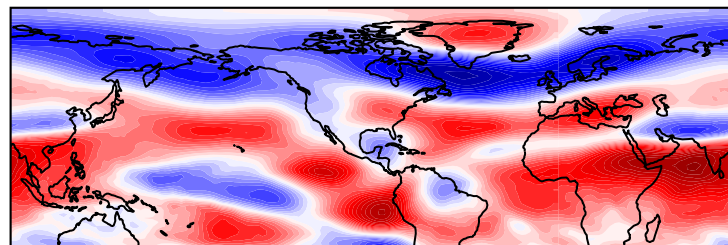
e) U200 SHAP - Winter - Week 2 Greenland High - # Correct cases: 77
