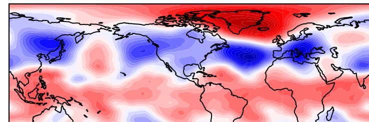
f) Z500 SHAP - Fall - Week 2 Greenland High - # Correct cases: 40
