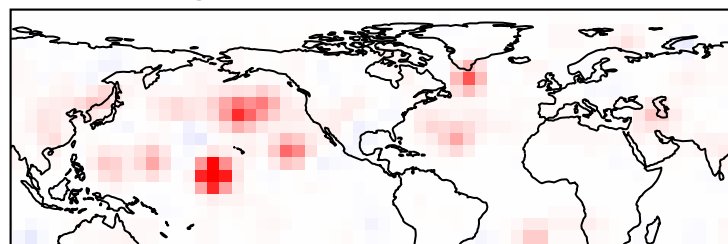
k) Z500 SHAP - Fall - Week 5 Pacific Trough - # Correct cases: 118
