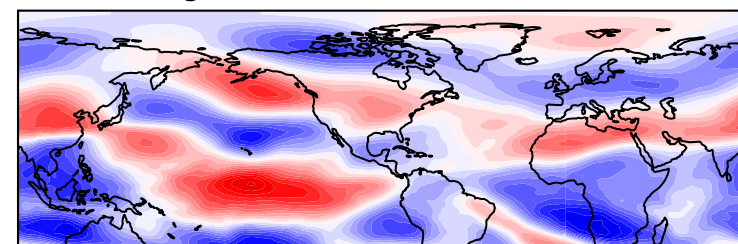
i) U200 Anoms. - Winter - Week 5 Pacific Ridge - # Correct cases: 93
