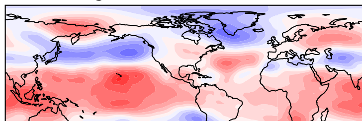
h) Z500 Anoms. - Fall - Week 5 Pacific Trough - # Correct cases: 118
