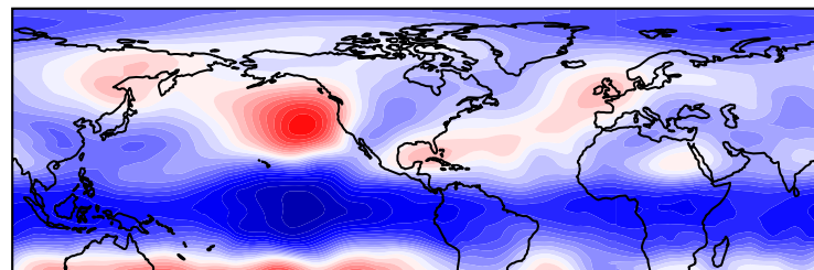
d) Z500 SHAP - Winter - Week 3 Pacific Ridge - # Correct cases: 91
