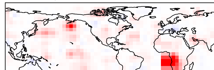
l) U200 SHAP - Winter - Week 5 Pacific Ridge - # Correct cases: 93
