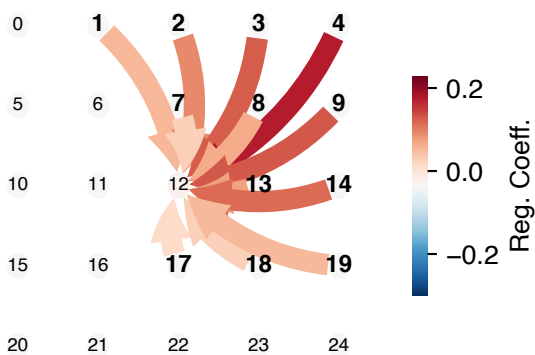
B. Elastic-Net: V_1(t-1) \rightarrow V_1(t) causal parents
