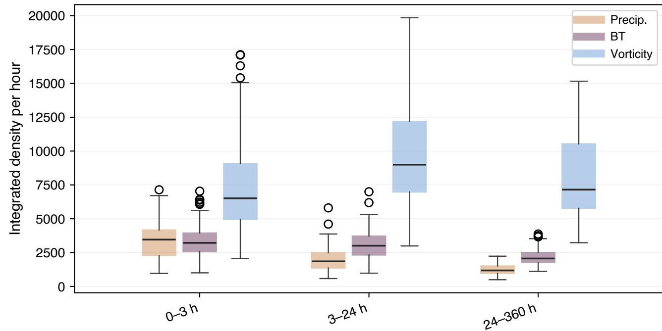
Debby: causal relevance by backward-time window
