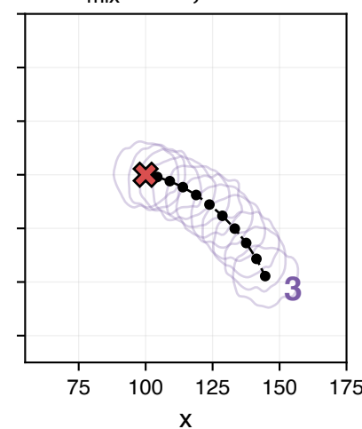
M. \alpha_{\text{mix}} = 0.8 , Var. 3
