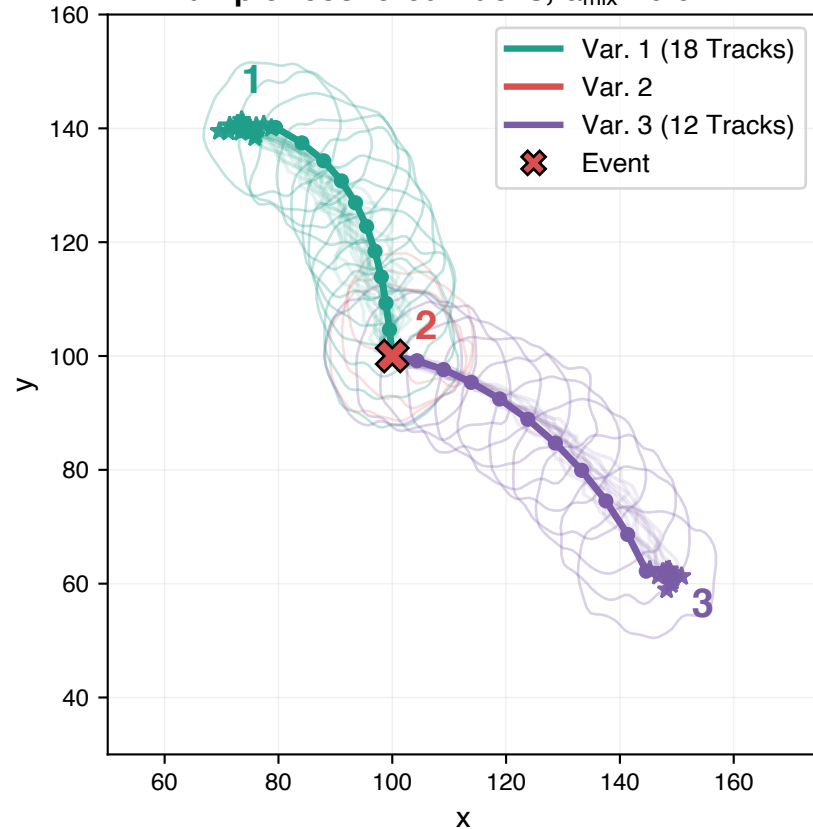
H. Example recovered tracks, \alpha_{\text{mix}} = 0.6
