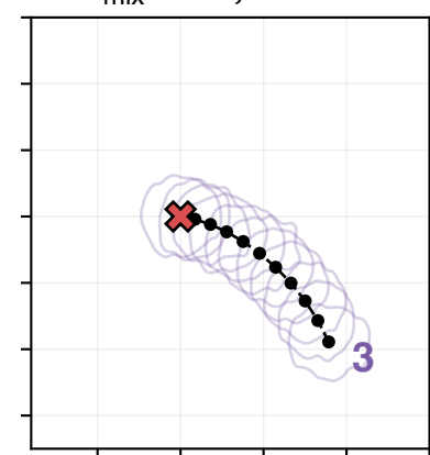
M. \alpha_{\text{mix}} = 0.8 , Var. 3
