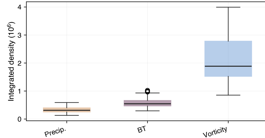
F. Mid-level vorticity
