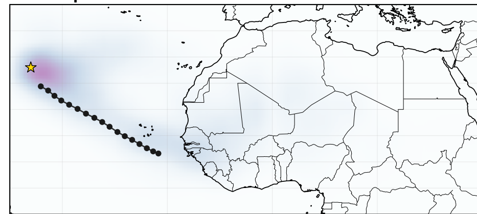
D. Precipitation
