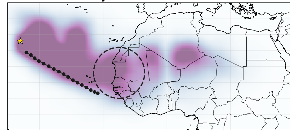
F. Mid-level vorticity
