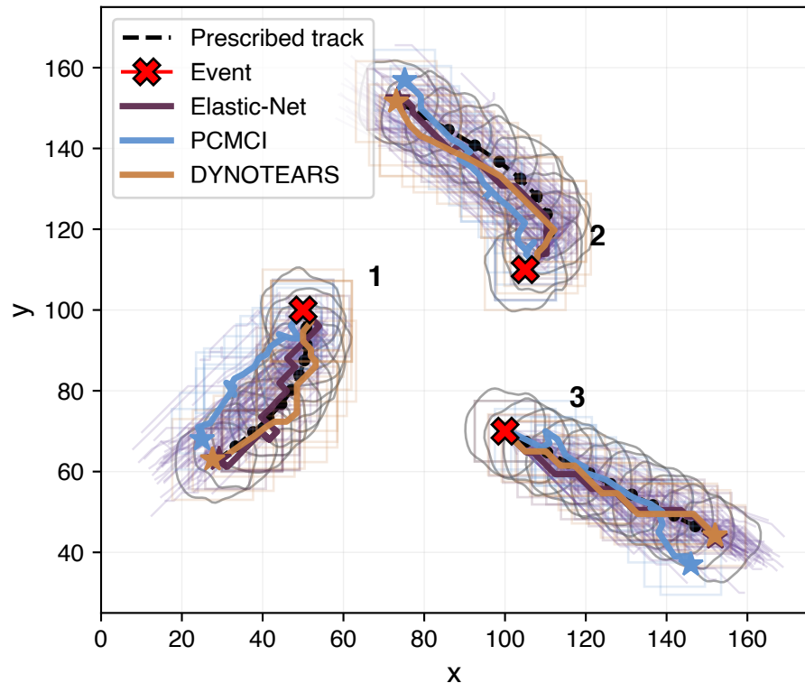
A. Prescribed and recovered tracks
