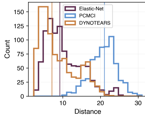
F. Mean track distance
