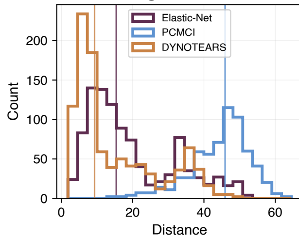
E. Mean origin distance
