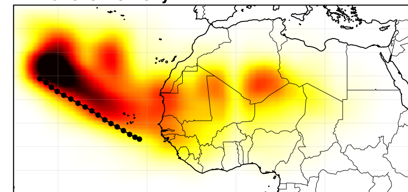
F. Mid-level vorticity
