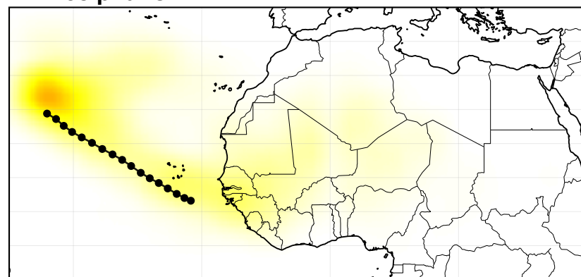
D. Precipitation
