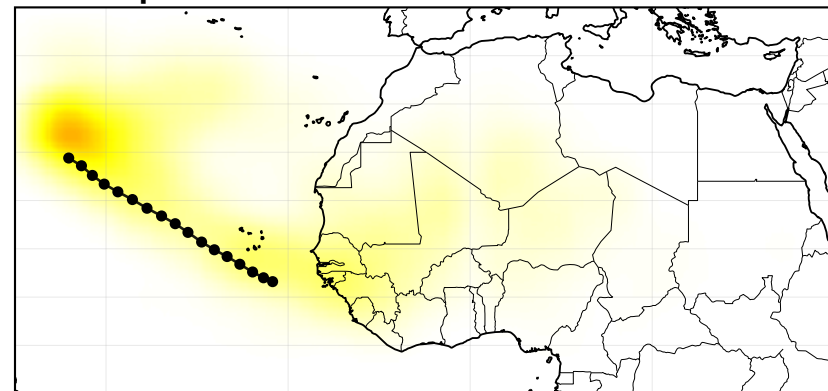
D. Precipitation
