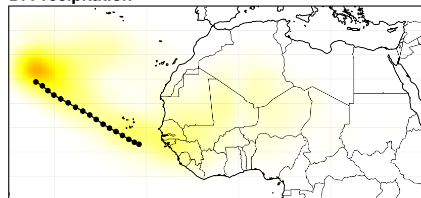
D. Precipitation
