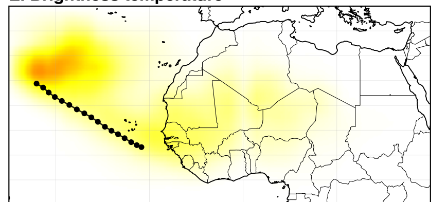
E. Brightness temperature
