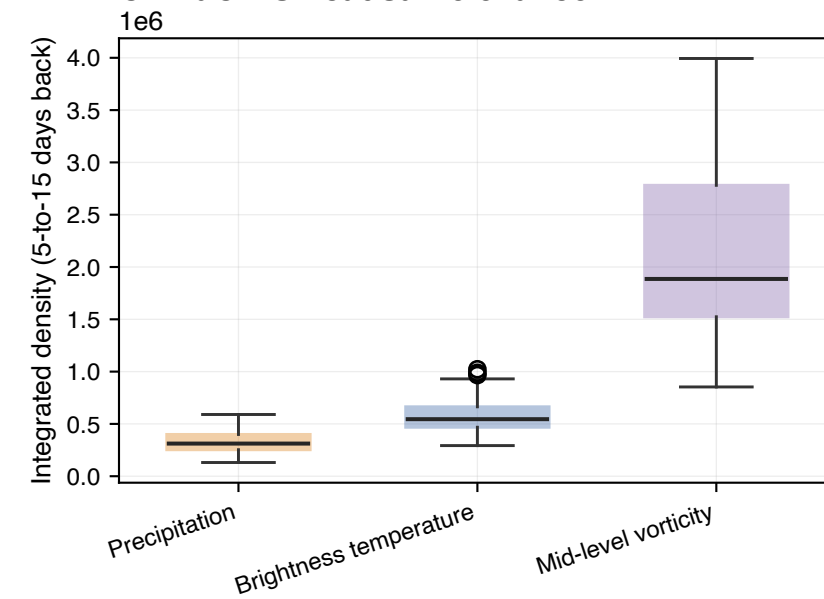
F. Mid-level vorticity
