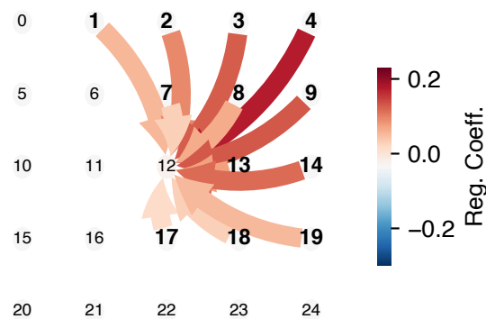
B. Elastic-Net: V_1(t-1) \rightarrow V_1(t) causal parents
