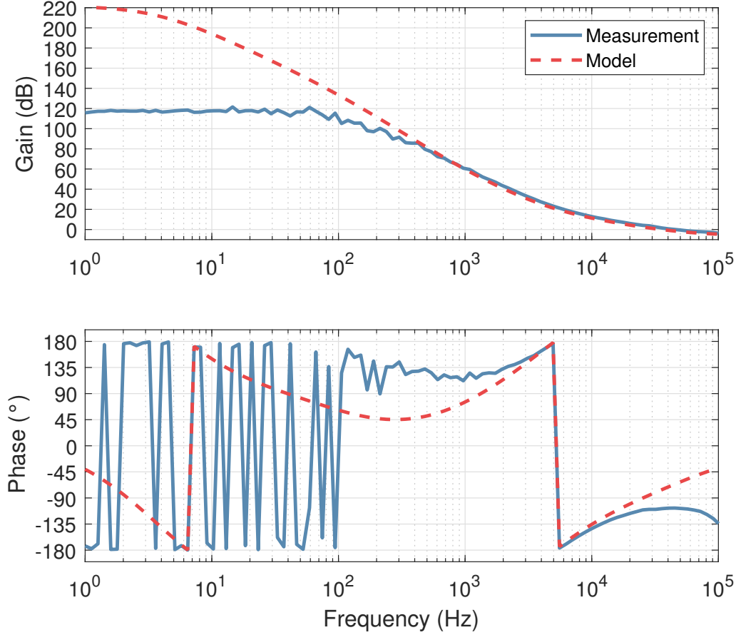
Figure 2.19: The open-loop transfer function was measured using the layout shown in Figure 2.18. The unity gain point is at 48 kHz with 70° of phase margin. The shaping of the servo is 1/f at the unity gain point, but to achieve higher gain at low frequency, the servo has a 1/f^3 slope between 10 Hz—5 kHz. The measurement saturated below 100 Hz. The model and measurement do not agree well below a few kHz due to the measurement saturating.
