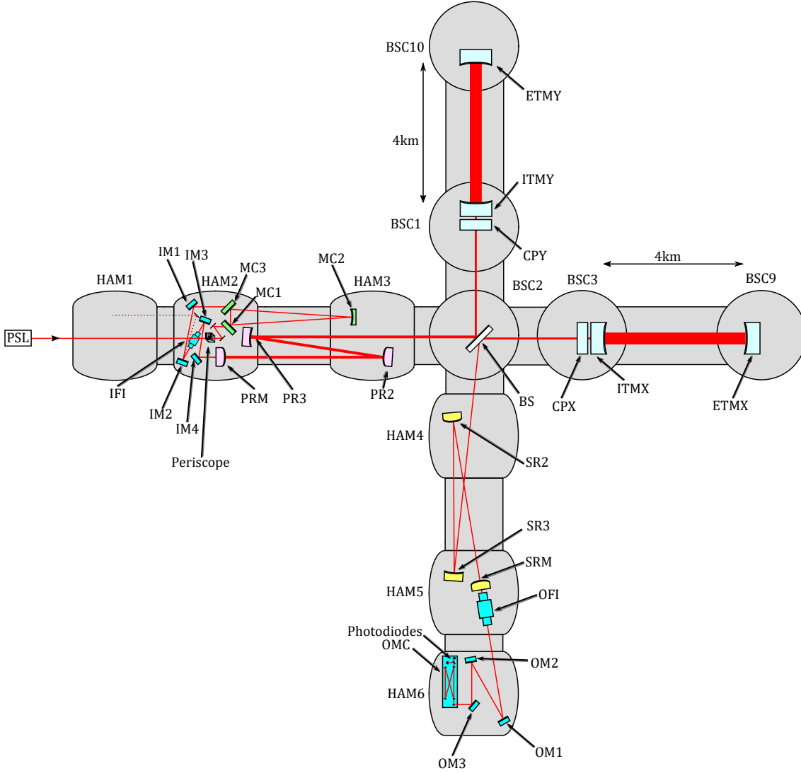
Figure 1.4: Sketch of a LIGO detector. The input and output optics — IM1-4, the input periscope, OM1-3, the OMC, the input Faraday isolator and the OFI — are shown in blue. The input mode cleaner mirrors are shown in green. The power recycling mirrors are shown in pink. The arm cavity mirrors are shown in pale blue. The signal recycling cavity mirrors are shown in yellow. The beam leaves BS at an angle due to the BS being wedged. Angles in the recycling cavities are exaggerated and the arms are shortened for clarity.
