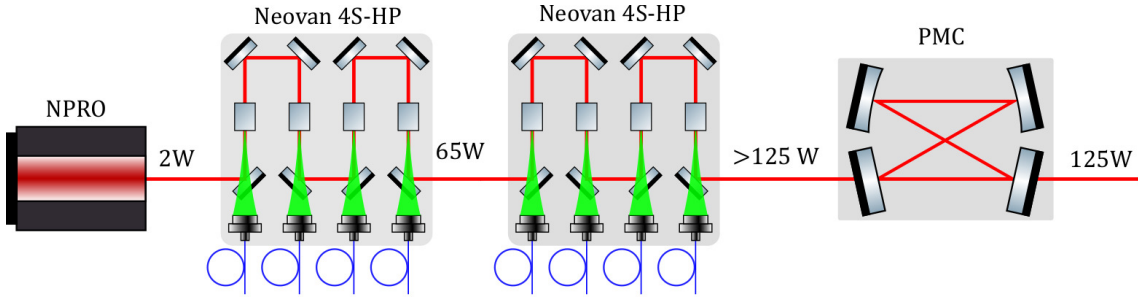
Figure 2.1: Conceptually, the PSL will be made up of four components: the NRPO, two neoVAN-4S-HP amplifiers and the PMC cavity. The NPRO provides seed light with good noise characteristics. These noise characteristics are preserved by the amplifiers, so the resulting beam will have high power and low noise. As the linewidth of the PMC \sim 1 MHz, it filters away light in higher order modes and RF intensity noise so a quiet spatially pure mode can be sent to the interferometer.
