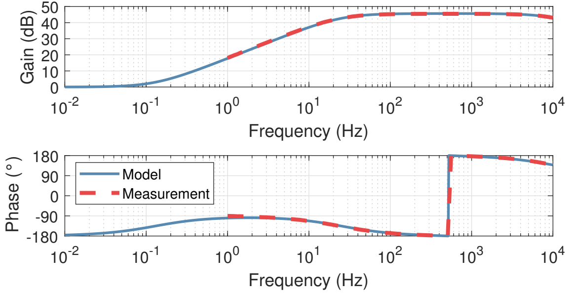
Figure 7.4: The transfer function of the electronics for sending, receiving and whitening the photodiode signal was modelled and measured. This gave the desired level of SNR to make shot noise limited measurements above \sim 200 Hz.
