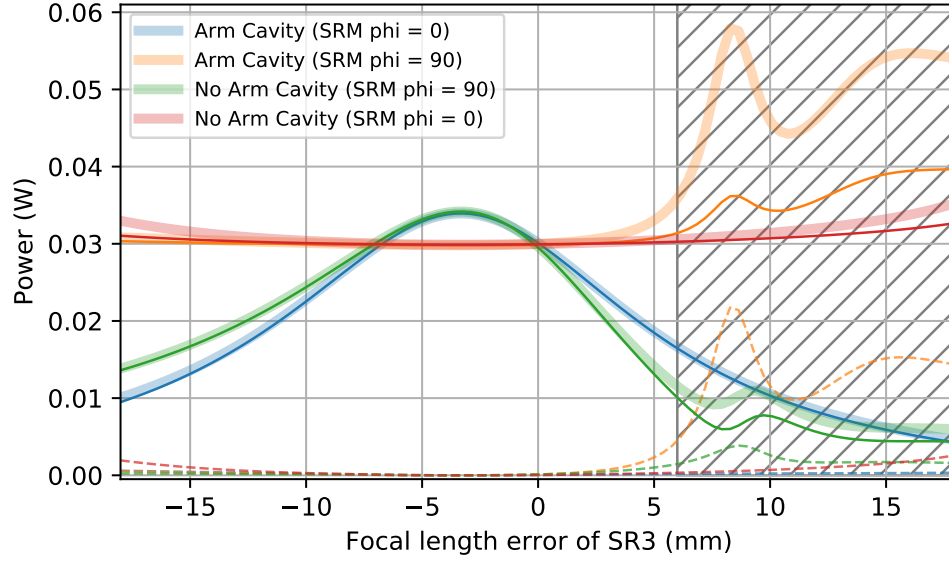
Figure 4.14: The total power transmitted through the SRM for each simulation, is shown in the thick pale lines. The thin solid lines corresponds to the power in the HG00 mode, and the thin dashed lines correspond to the power in the higher order modes. Blue lines show the behaviour when the interferometer has arm cavities and is in signal recycling mode, and the orange lines shows when it is in RSE mode. Green lines show how the power changes when the interferometer is configured for a single bounce measurement and is in signal recycling mode, and the red line shows when its in RSE mode. The hatched region indicates where the SRC is becomes unstable, and so the behaviour of the interferometer cannot be accurately simulated for these values of focal length.
