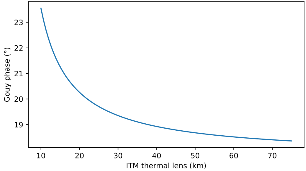
Figure 4.9: Gouy phase between the ITMs and the SRM as a function of the thermal lens in the ITMs for nominal values of SR3 and SR2. The nominal ITM thermal lens is 50 km, and this corresponds to about 19°. More heating results in a greater thermal lens, however the LIGO detectors compensate for this with the thermal compensation system (TCS).
