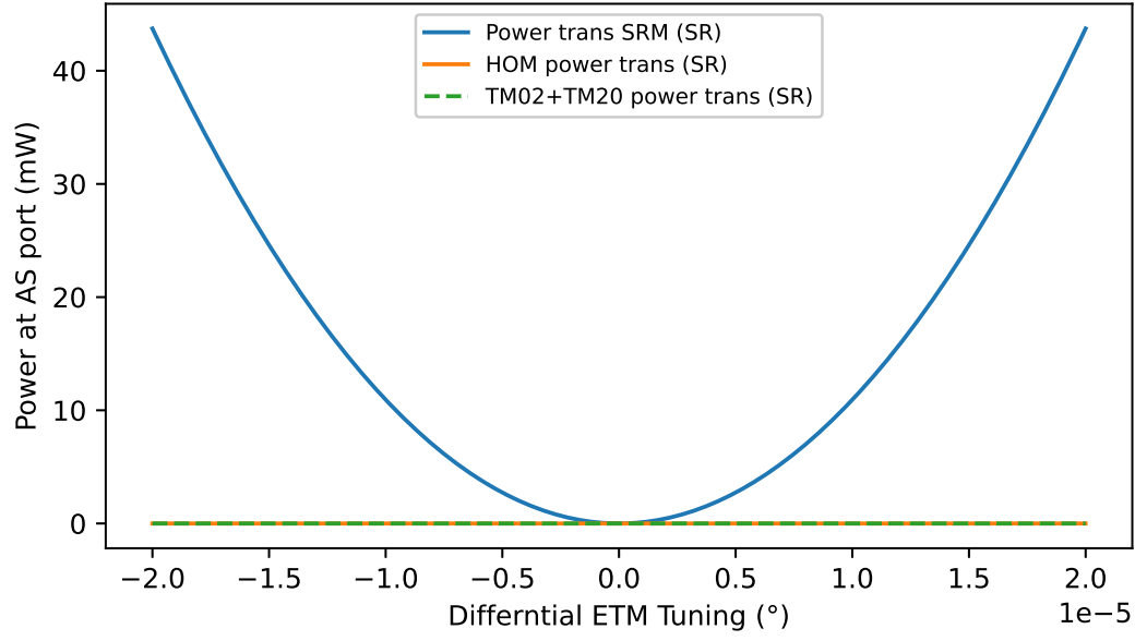
Figure 4.4: The minimum of the dark fringe is at 0^\circ differential ETM detuning, as shown by the blue line. A slight offset causes light to be as the AS port. This result was used to determine tunings for simulating what effect focal length errors in SR3 and SR2 have on the beam transmitted through the SRM. The orange and green dashed line show the HOM content of the beam.
