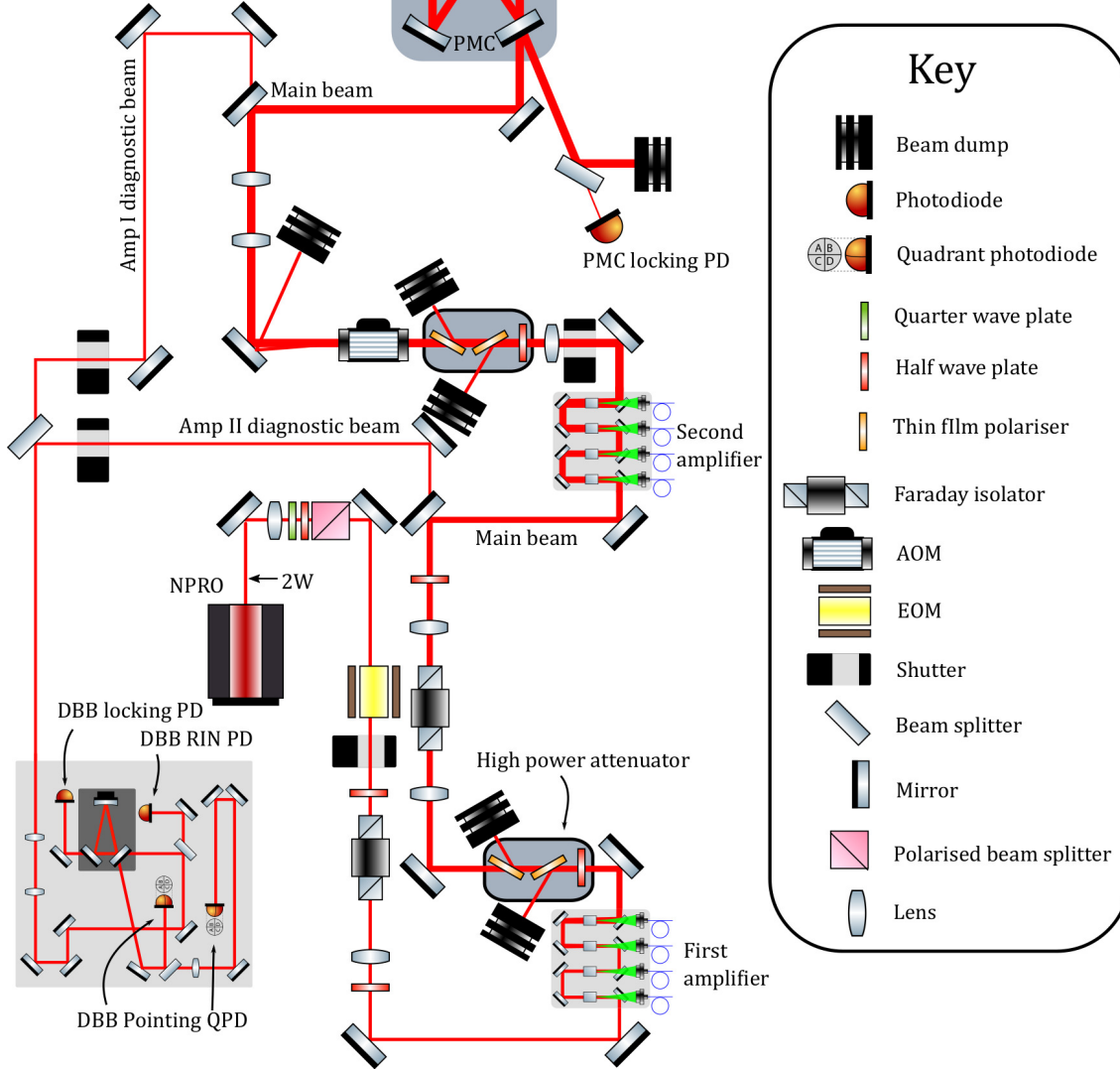
Figure 3.2: Sketch of the prototype optical layout for the PSL. The main and diagnostic beam paths are shown. This sketch shows all the optics in the main beam path as well as the pick-off points for the diagnostic beams.
