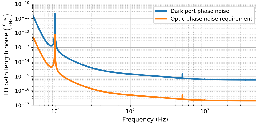
Figure 5.5: The sensitivity curve for A+ sets the limit on how much path length noise is acceptable between the AS and LO beams. The blue line shows sensitivity curve in units of path length noise between the AS and LO beams, and the orange line shows the longitudinal motion requirement for the optics which combine the LO and signal beam. At 5 Hz, the longitudinal motion requirement for the optics is 4.9 \times 10^{-13} \text{ m}_{\text{rms}}/\sqrt{\text{Hz}} . The red line shows the level of shot noise; this is 2.1 \times 10^{-17} \text{ m}_{\text{rms}}/\sqrt{\text{Hz}} .
