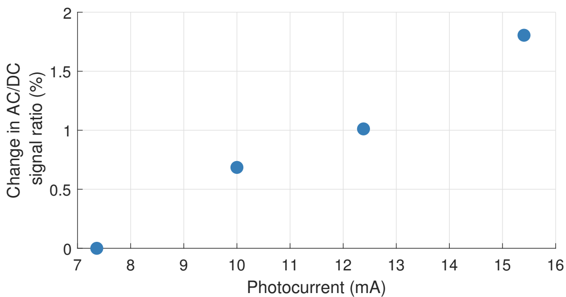
Figure 8.4: The bias of the FD10D was set to 0.6 V, and it was exposed to a series of different power levels to check at what photocurrent the photodiode would saturate at. This was done by measuring the height of the calibration peak; if this peak decreased in size relative to the DC signal then this would indicate the photodiode was saturating. This peak could only be measured to within 1%, and so the FD10D showed no sign of saturation under these conditions.
