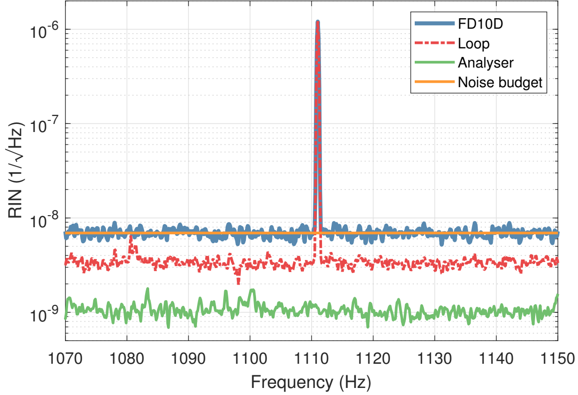
Figure 8.3: The bias of the FD10D was set to 0.6 V, and it was exposed to 15 mW of 1.55\text{ }\mu\text{m} light. 15 mA of photocurrent was generated. The noise of the photocurrent produced by the FD10D (blue line) corresponds to the level predicted by Equation 8.3 (orange line) meaning that the increase in photocurrent can only be explained by an increase in quantum efficiency. The 1111 Hz signal was used to calibrate the measurement as this modulation also could be measured on the high-performance in-loop photodiode.
