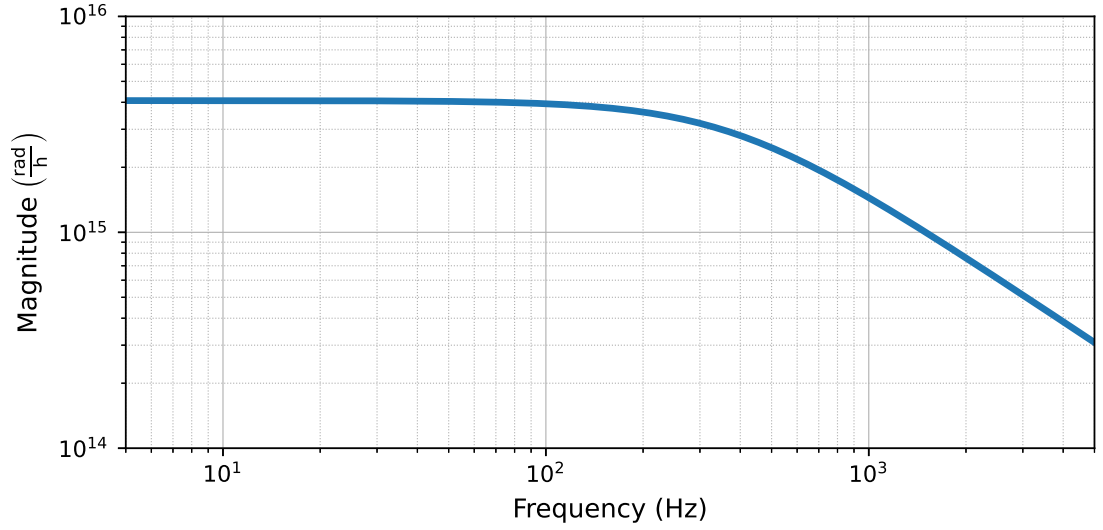
Figure 5.3: The linear response function between strain and light power, expressed in units of radians/gravitational wave strain, at the AS port. The corner frequency at \approx 380 Hz comes from the pole of the coupled SRC-arm cavity.
