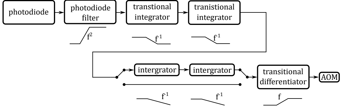
Figure 3.21: Block diagram of the components in the the intensity stabilisation servo. The transfer function of each block is described in Section 3.5.4.1 and Table 3.1. The overall gain of the servo depends on a variable gain chip and the amount of light on the photodiode. The shaping of each block is indicated below it.
