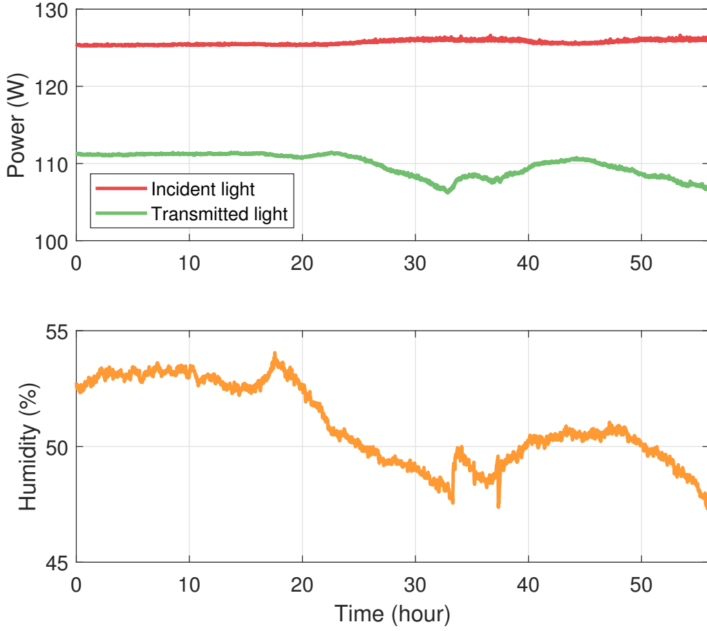
Figure 3.7: The top panel shows the power that was incident on the PMC and the power emerging from the PMC over a 55 hour trial run. The light produced by the amplifiers did not change significantly for the duration of this measurement, however the transmitted light through the PMC dropped from 111 W to, at its lowest, 107 W. This is likely due to the environmental conditions in the lab changing. The bottom panel shows the humidity of the lab. Changes in the humidity, which can be caused by a temperature change, coincide with changes in the power emerging from the PMC. This indicates that the alignment or mode matching of the laser and the PMC may be dependent on temperature due to e.g. the thermal expansion of optical mounts.
