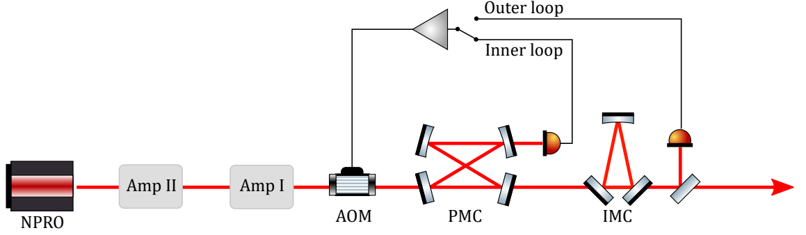
Figure 3.12: The intensity stabilisation concept involves two loops. The inner-loop is responsible for stabilising the laser so that the IMC can lock. The outer-loop is used to stabilise the laser for observation mode. The two loops sense the laser intensity noise at different points. The inner-loop uses a low power beam, \sim 1 mW, transmitted by the PMC. The outer-loop uses a higher power, \sim 350 mW, pick-off from the main beam. An AOM is used to actuate on the laser's power.
