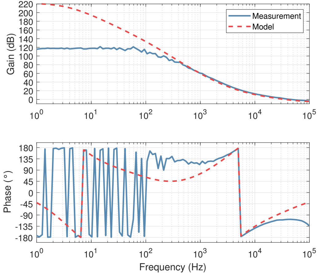
Figure 3.20: The open-loop transfer function was measured using the layout shown in Figure 3.19. The unity gain point is at 48 kHz with 70^\circ of phase margin. The shaping of the servo is 1/f at the unity gain point, but to achieve higher gain at low frequency, the servo has a 1/f^3 slope between 10 Hz—5 kHz. The measurement saturated below 100 Hz. The model and measurement do not agree well below a few kHz due to the measurement saturating.
