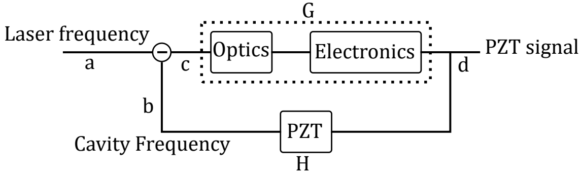
Figure 3.25: The servo can be considered as being made of three parts: the optics, the shaping electronics and the PZT. The transfer function of the optics represents how a difference in frequency between the laser and the cavity transforms into a signal after the demodulator. When at resonance and below the cavity pole, this is a flat transfer function that is proportional to the difference in frequency. Since this cavity pole is in the 1 MHz region and this measurement will only go to the kHz region, the cavity pole can be ignored. The transfer function of the electronics includes everything after the demodulator up to and including the final high power op amp. The PZT transfer function converts a voltage to a cavity frequency. The PZT has capacitance, so a low pass filter is formed by this and the series resistor at the output of the electronics.
