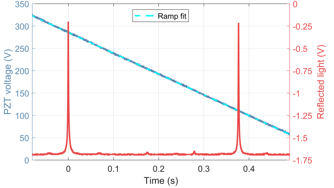
Figure 3.27: A ramp was applied to the PZT and the reflected light from the cavity was measured. The FSR of the cavity is known, so the time in this measurement can be converted to frequency. This gives the PZT transfer function at low frequencies. The ramp signal is shown in blue and the reflected light is shown in red.
