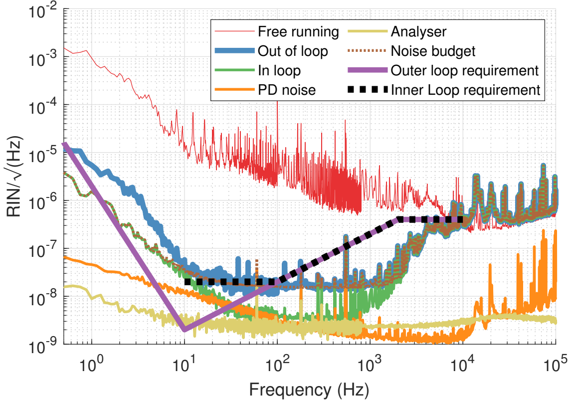
Figure 3.22: The free-running noise of the laser is shown in red. The noise of the light transmitted by the PMC is shown in blue; this meets the requirement that is shown by the dashed black line. The noise level is determined by the in loop noise, shown in green, the shot noise and other technical noise sources; the sum of these is shown by the dotted brown line. Between 10 Hz–100 Hz, the noise of the laser is limited by shot noise. There is a discrepancy between the noise budget and the measured noise. This is likely due to dust falling through the beam or scattered light. Near the unity gain point of the servo, the noise is enhanced by the servo due to gain peaking.
