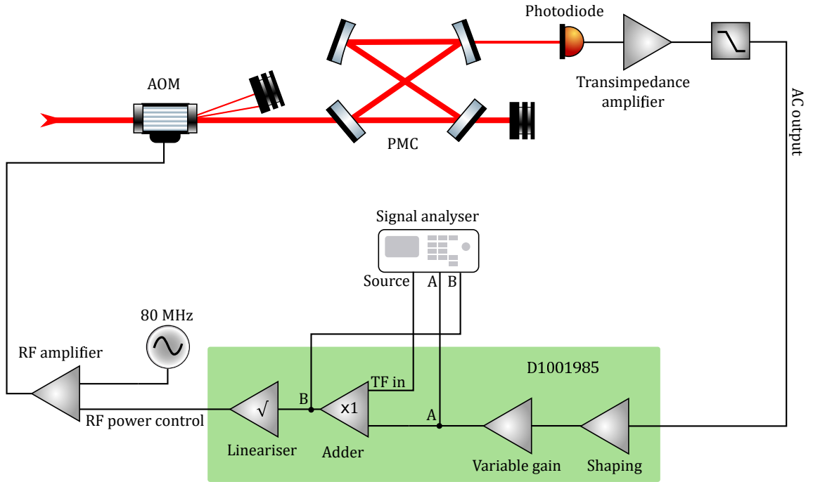
Figure 3.19: Sketch of the amplitude stabilisation servo. By measuring the ratio of the signal at point B and point A, the transfer function of all the parts in the servo (apart from the \times 1 adding stage) can be measured (see Figure 3.18).
