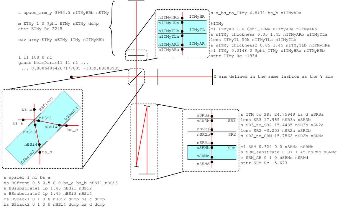
Figure 4.3: Schematic of the simulation. The dimensions of the schematic are not to scale. The laser light is shown as a red line. Black lines with red beams interacting with them correspond to components such as mirrors and lenses. Important nodes are highlighted with black dots and the associated FINESSE commands are shown nearby. Zoom-ins provide more detail for the main beam splitter, ITMy and the SRC. The elongated curled bracket highlights the arm cavity, and the text with it shows how it is implemented in FINESSE.
