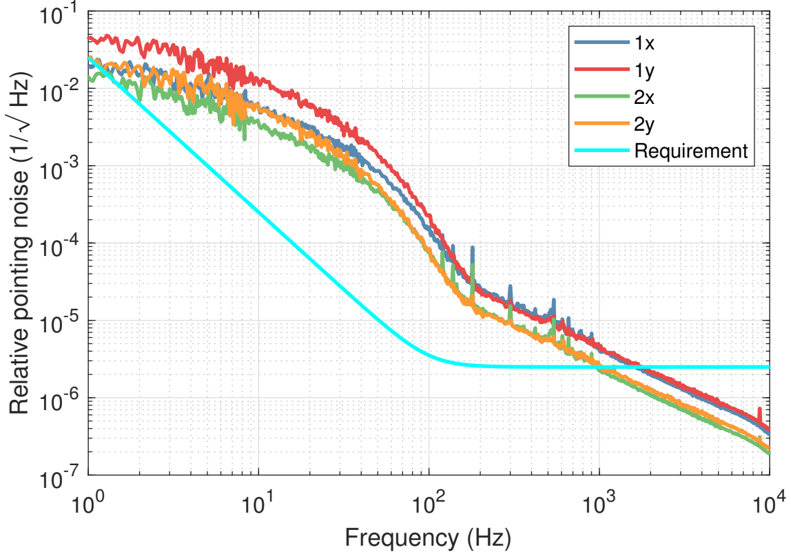
Figure 3.23: The four relative pointing degrees of freedom for the beam into the PMC was measured with the DBB. The requirement [128] is shown in light blue. The pointing noise is above the requirement, however the TnT lab has a higher amount of environmental noise than the PSL. Measurements below 200 Hz were be affected by scattering.
