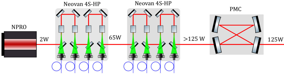
Figure 3.1: Conceptually, the PSL will be made up of four components: the NRPO, two neoVAN-4S-HP amplifiers and the PMC cavity. The NPR0 provides seed light with good noise characteristics. These noise characteristics are preserved by the amplifiers, so the resulting beam will have high power and low noise. As the linewidth of the PMC \sim 1 MHz, it filters away light in higher order modes and RF intensity noise so a quiet, spatially pure mode can be sent to the interferometer.
