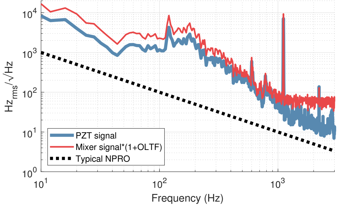
Figure 3.29: The mixer signal combined with the open-loop transfer function is shown in red. This is equivalent to the frequency noise of the system. The PZT signal should agree with this measurement below the unity gain point ( \sim 800 Hz). A signal was applied to the PZT at 1111 Hz. This is below the corner frequency of the PZT and above the unity gain point for the servo. This should match with the mixer signal. There is a factor of two between these two measurements. This can be attributed to imperfect calibration due to nominal parameters of the PMC being used. The typical noise expected from an NPRO is shown by the dashed black line. Between 100 Hz and 1000 Hz, there is a bulge in the frequency noise. This is likely due to acoustically driven noise of the PMC as the PMC is not vacuum sealed. This can be converted to length noise with a factor of \sim 10^{-14} m/Hz.
