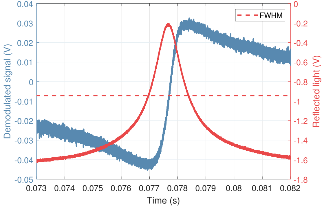
Figure 3.26: A ramp was applied to the PZT and the photodiode signal was measured before and after demodulation. The demodulated photodiode signal is shown in blue. The photodiode signal is shown in red. Around the peak of the photodiode signal, the slope of the demodulated signal gives the gain of the ‘optics’ transfer function. This can be expressed in units of V/MHz by converting the time axis to a frequency axis. This is done by using the FWHM of the photodiode signal as a reference frequency. The level of the FWHM is indicated by the dashed red line.
