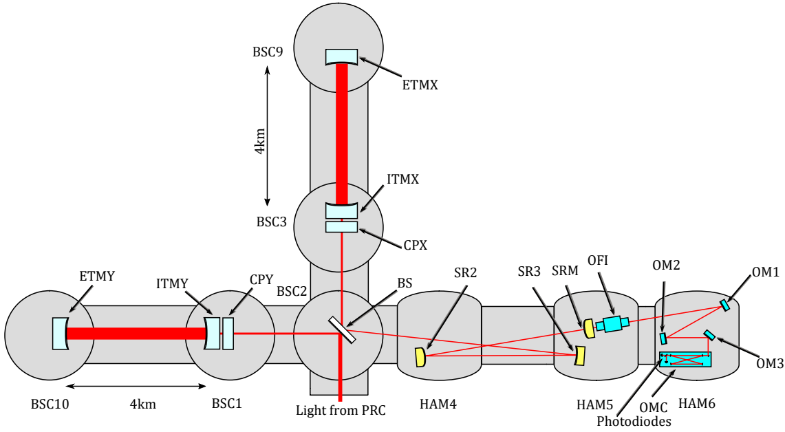
Figure 4.1: Sketch showing the parts of the aLIGO detectors discussed in this chapter. A more complete sketch is shown in Figure 2.4. The angles and lengths are exaggerated for clarity. Light from the arm cavities is incident upon the beam splitter (BS). As BS is wedged, the light going towards the SRC comes out at an angle. Differential arm length signals encoded onto this light are directed towards SR3, SR2, and then the SRM. Between the SRM and the OMC, there are optics for steering and mode matching (OM1-3). Finally, to strip away junk light, the light enters the OMC. The light emerging from the OMC is detected by photodiodes.
